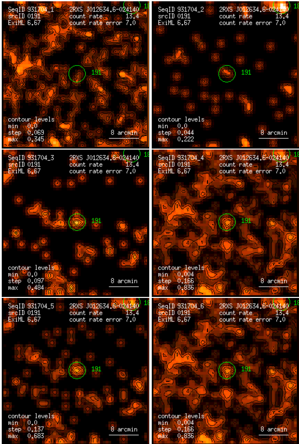
Figure 191: RASS 931704: detection 0191: band rate images, Gaussian filter: (1) PSPC channels 11 – 41, (2) 52 – 90, (3) 91 – 201, (4) 11 – 235, (5) 52 – 201, (6) 11 – 201. Broad band rates in counts/ks. Band rate contour levels in counts/ks/arcmin 2 .
