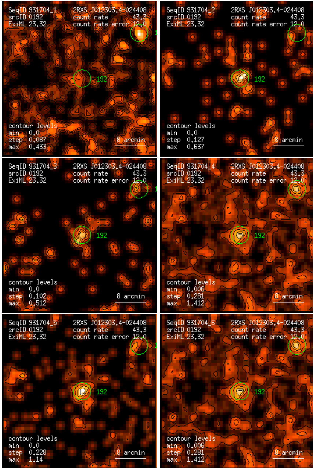
Figure 192: RASS 931704: detection 0192: band rate images, Gaussian filter: (1) PSPC channels 11 – 41, (2) 52 – 90, (3) 91 – 201, (4) 11 – 235, (5) 52 – 201, (6) 11 – 201. Broad band rates in counts/ks. Band rate contour levels in counts/ks/arcmin 2 .
