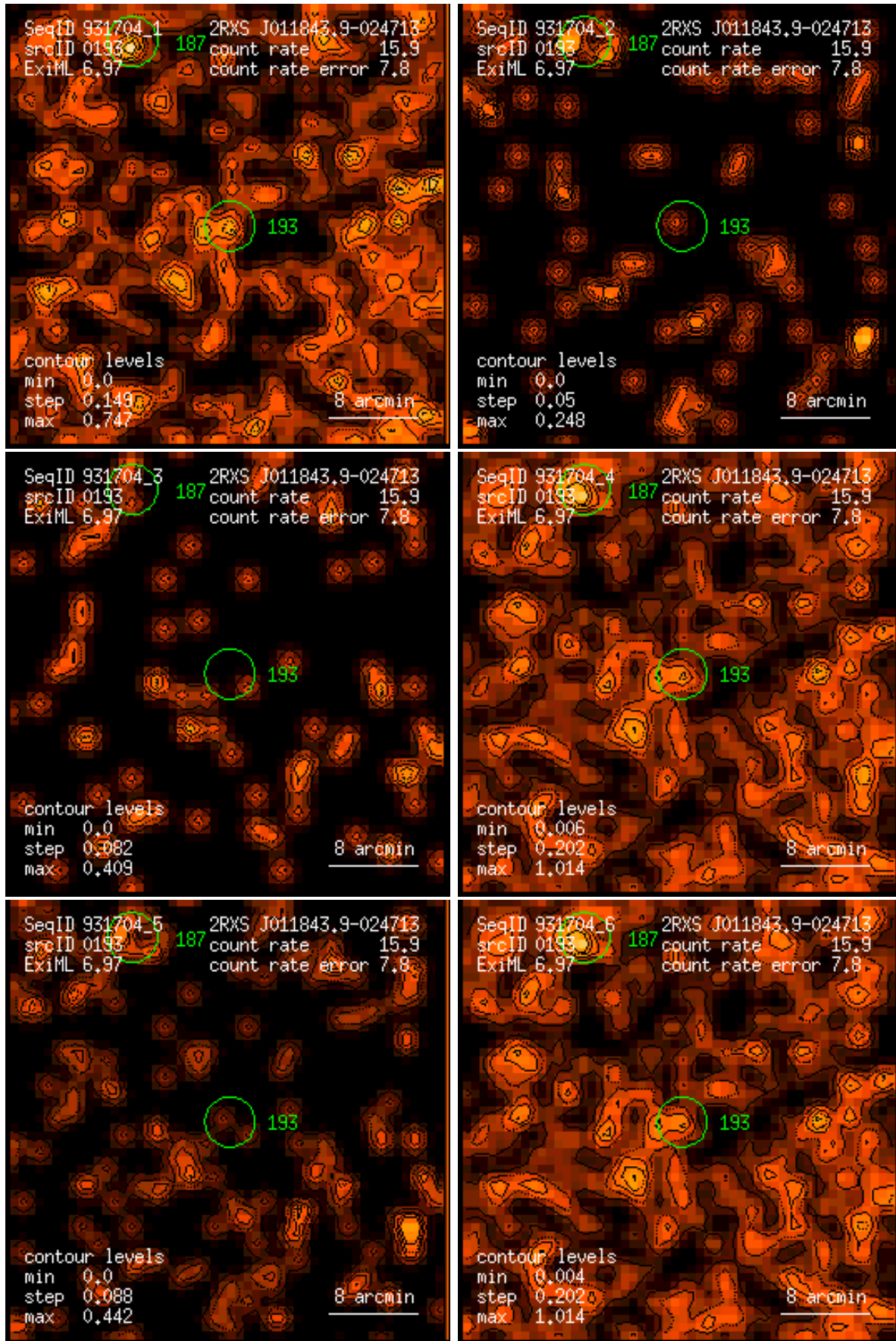
Figure 193: RASS 931704: detection 0193: band rate images, Gaussian filter: (1) PSPC channels 11 – 41, (2) 52 – 90, (3) 91 – 201, (4) 11 – 235, (5) 52 – 201, (6) 11 – 201. Broad band rates in counts/ks. Band rate contour levels in counts/ks/arcmin 2 .
