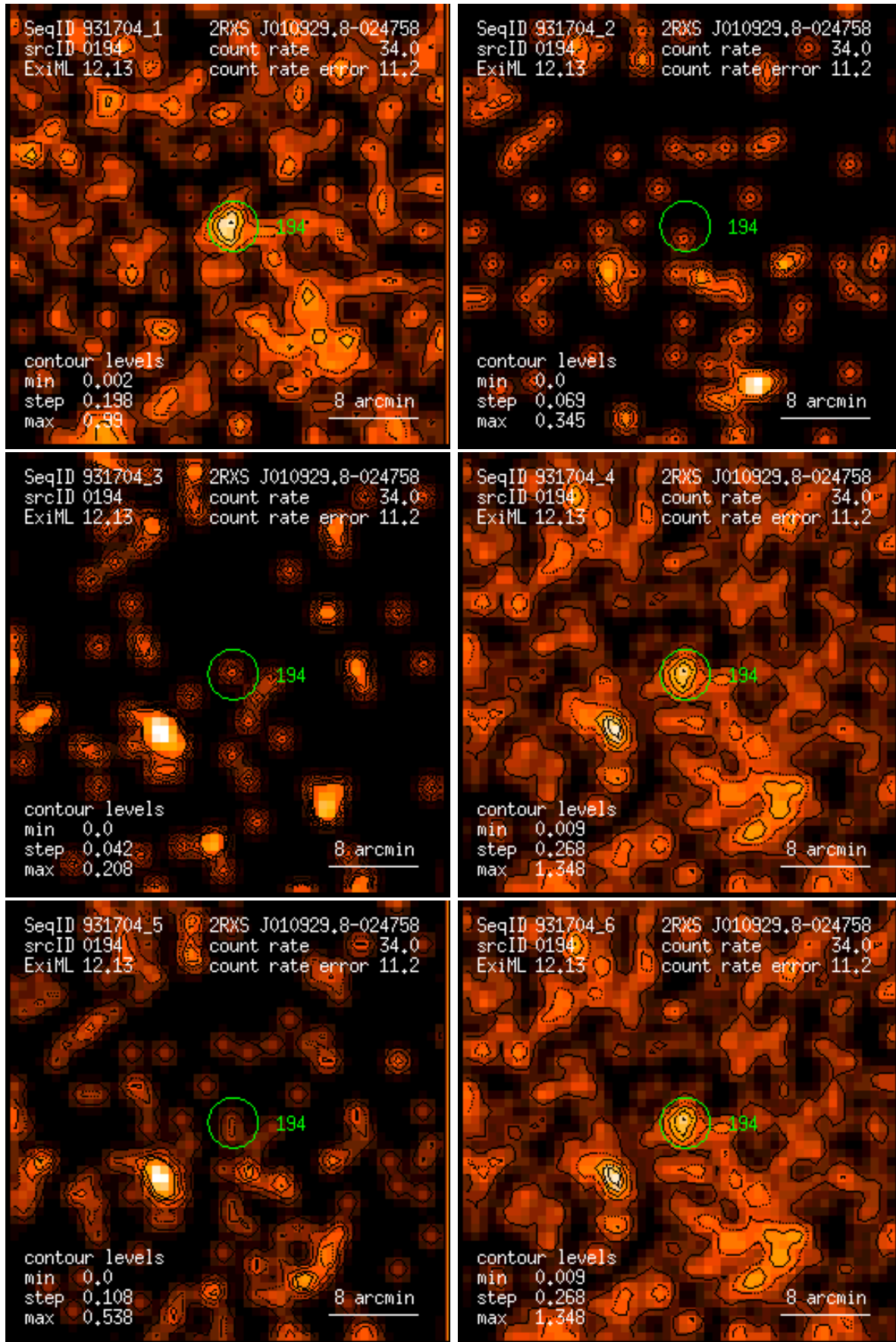
Figure 194: RASS 931704: detection 0194: band rate images, Gaussian filter: (1) PSPC channels 11 – 41, (2) 52 – 90, (3) 91 – 201, (4) 11 – 235, (5) 52 – 201, (6) 11 – 201. Broad band rates in counts/ks. Band rate contour levels in counts/ks/arcmin 2 .
