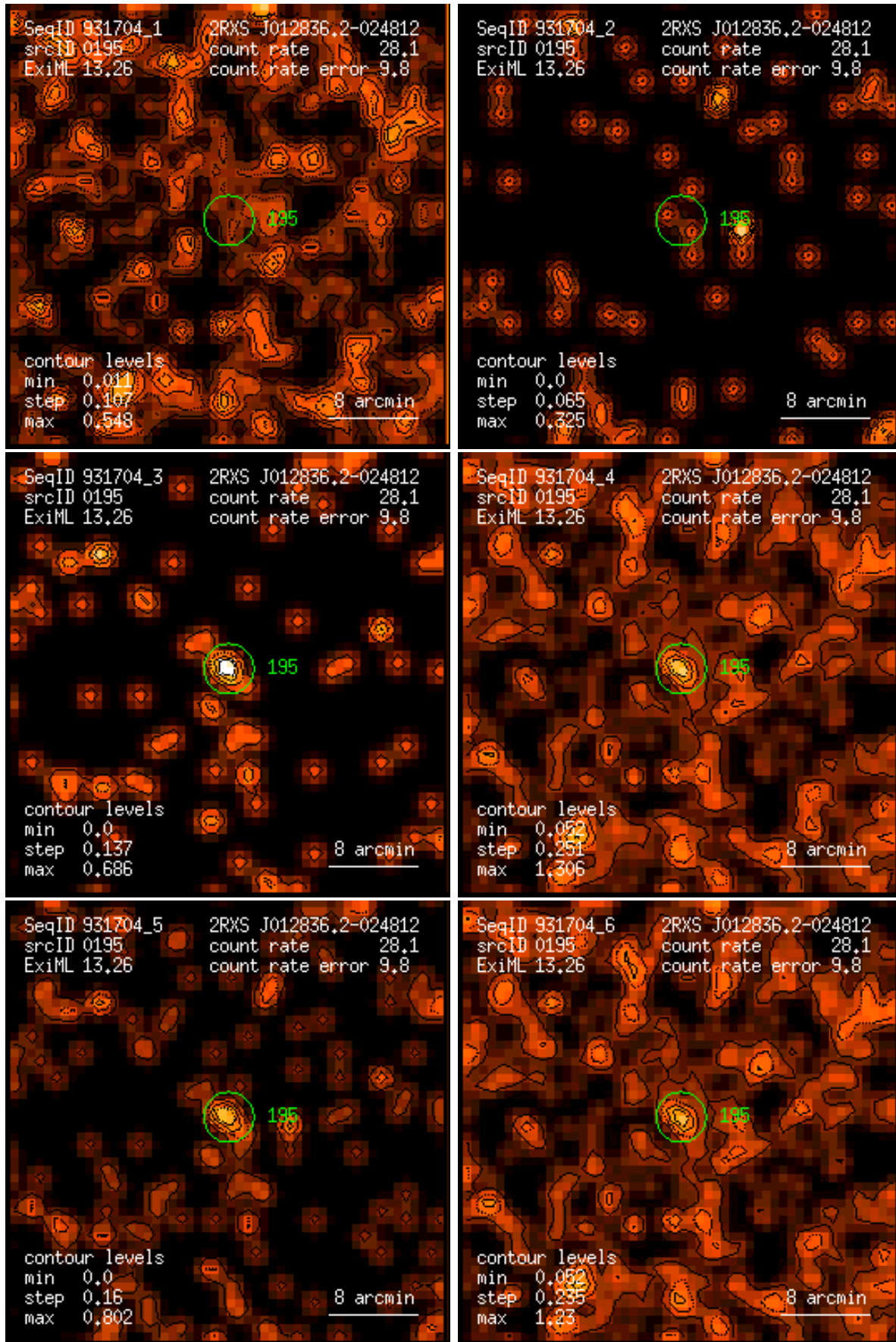
Figure 195: RASS 931704: detection 0195: band rate images, Gaussian filter: (1) PSPC channels 11 – 41, (2) 52 – 90, (3) 91 – 201, (4) 11 – 235, (5) 52 – 201, (6) 11 – 201. Broad band rates in counts/ks. Band rate contour levels in counts/ks/arcmin 2 .
