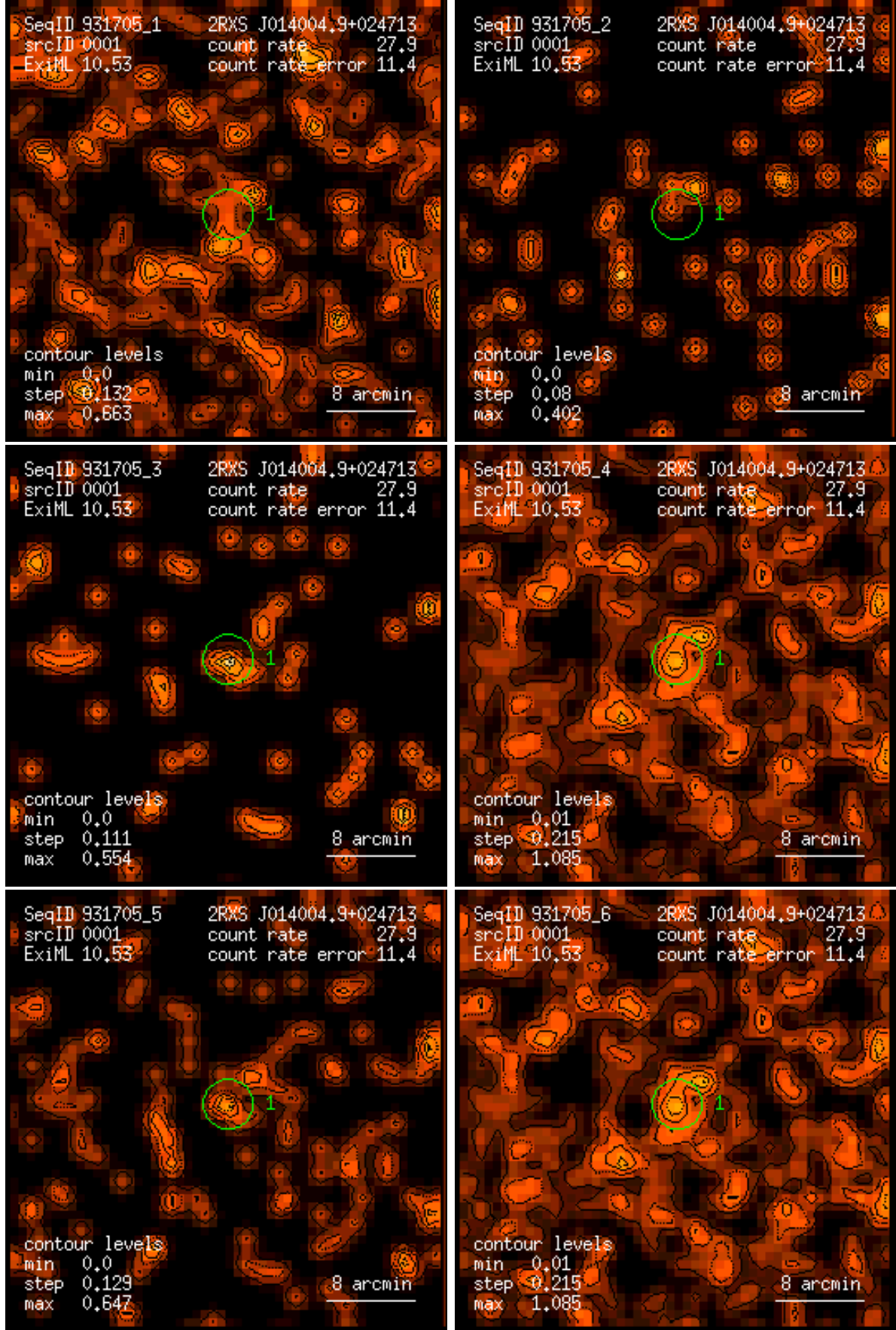
Figure 1: RASS 931705: detection 0001: band rate images, Gaussian filter: (1) PSPC channels 11 – 41, (2) 52 – 90, (3) 91 – 201, (4) 11 – 235, (5) 52 – 201, (6) 11 – 201. Broad band rates in counts/ks. Band rate contour levels in counts/ks/arcmin 2 .
