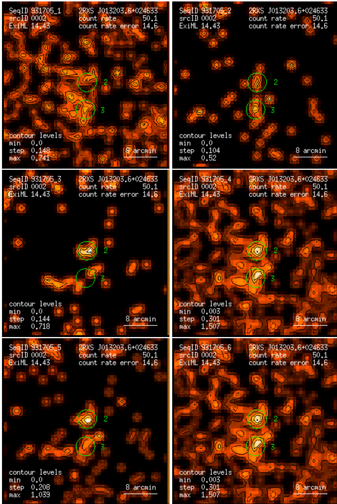
Figure 2: RASS 931705: detection 0002: band rate images, Gaussian filter: (1) PSPC channels 11 – 41, (2) 52 – 90, (3) 91 – 201, (4) 11 – 235, (5) 52 – 201, (6) 11 – 201. Broad band rates in counts/ks. Band rate contour levels in counts/ks/arcmin 2 .
