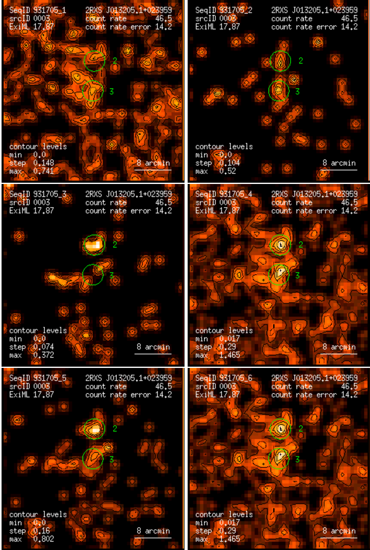
Figure 3: RASS 931705: detection 0003: band rate images, Gaussian filter: (1) PSPC channels 11 – 41, (2) 52 – 90, (3) 91 – 201, (4) 11 – 235, (5) 52 – 201, (6) 11 – 201. Broad band rates in counts/ks. Band rate contour levels in counts/ks/arcmin 2 .
