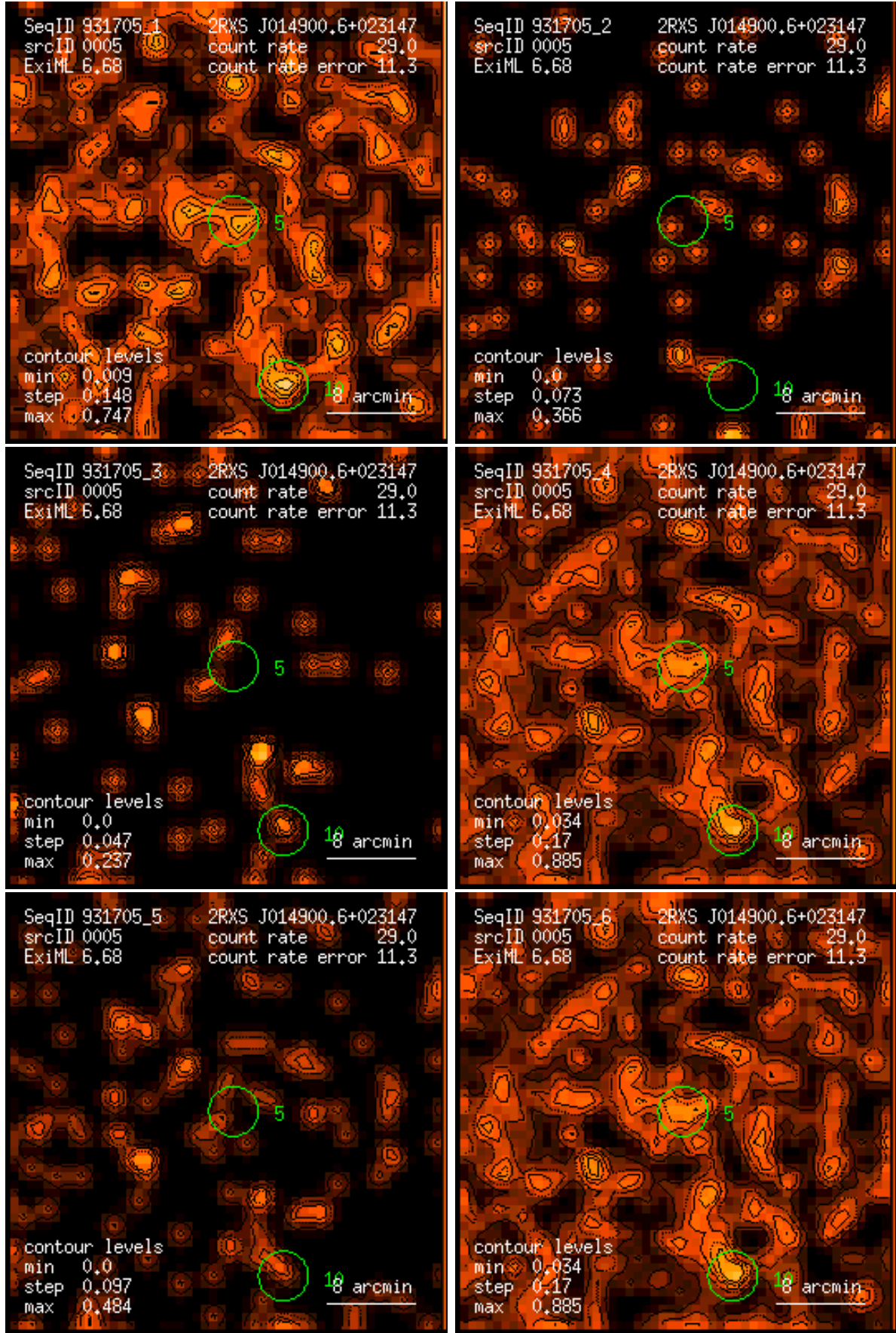
Figure 5: RASS 931705: detection 0005: band rate images, Gaussian filter: (1) PSPC channels 11 – 41, (2) 52 – 90, (3) 91 – 201, (4) 11 – 235, (5) 52 – 201, (6) 11 – 201. Broad band rates in counts/ks. Band rate contour levels in counts/ks/arcmin 2 .
