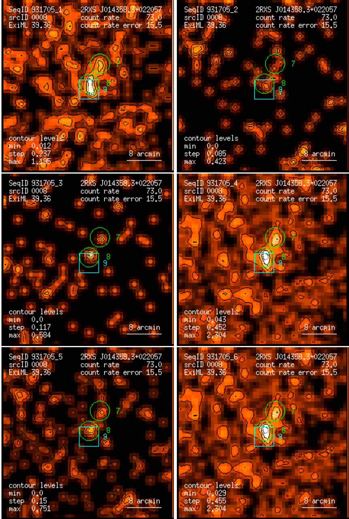
Figure 8: RASS 931705: detection 0008: band rate images, Gaussian filter: (1) PSPC channels 11 – 41, (2) 52 – 90, (3) 91 – 201, (4) 11 – 235, (5) 52 – 201, (6) 11 – 201. Broad band rates in counts/ks. Band rate contour levels in counts/ks/arcmin 2 .
