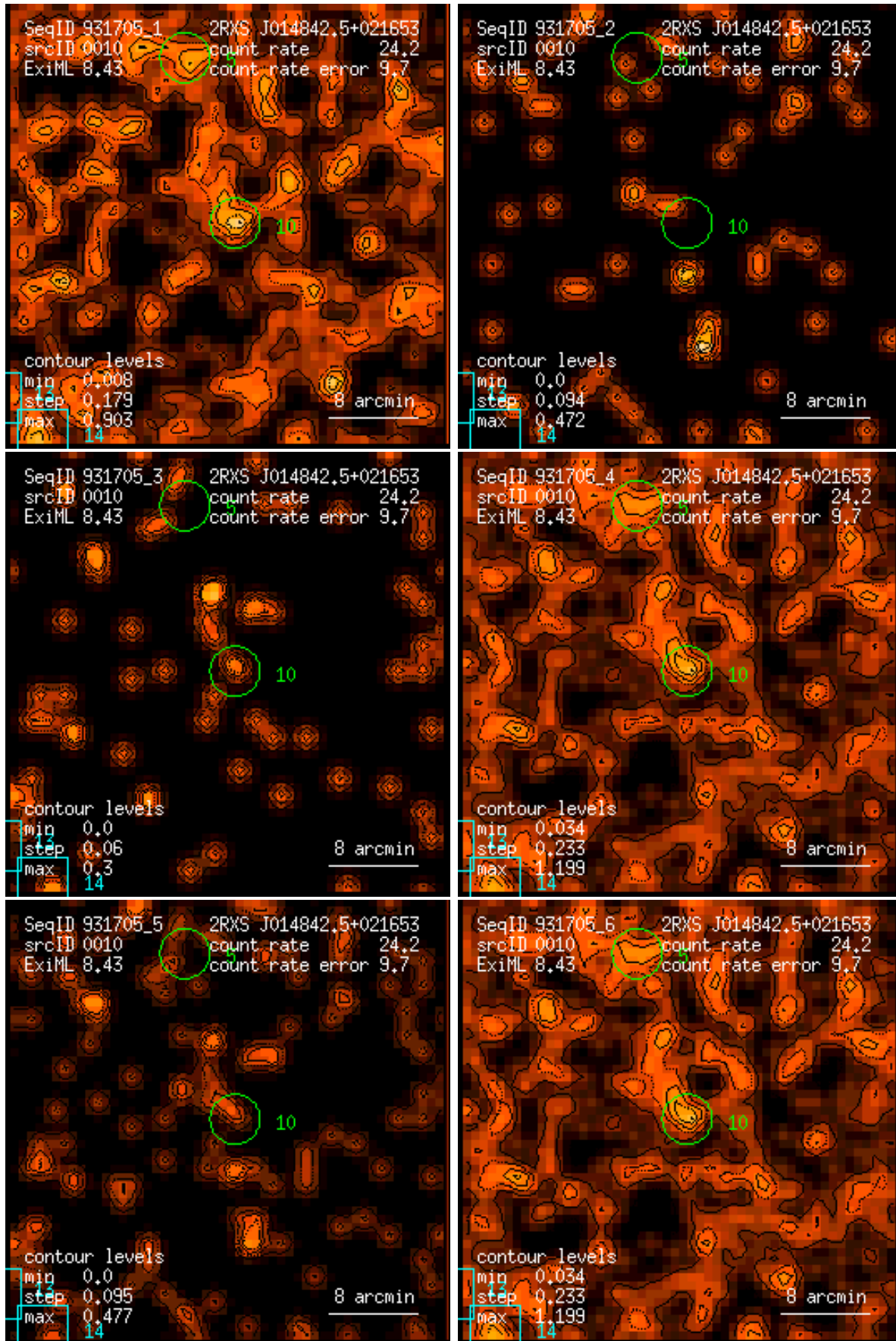
Figure 10: RASS 931705: detection 0010: band rate images, Gaussian filter: (1) PSPC channels 11 – 41, (2) 52 – 90, (3) 91 – 201, (4) 11 – 235, (5) 52 – 201, (6) 11 – 201. Broad band rates in counts/ks. Band rate contour levels in counts/ks/arcmin 2 .
