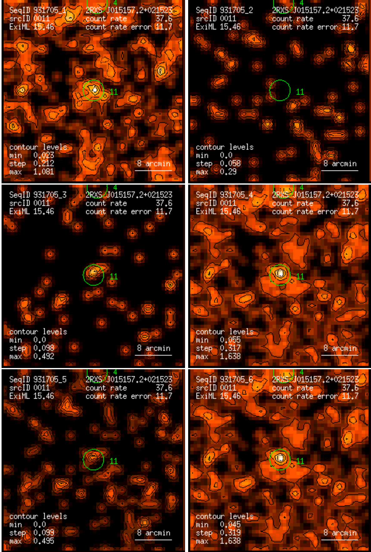
Figure 11: RASS 931705: detection 0011: band rate images, Gaussian filter: (1) PSPC channels 11 – 41, (2) 52 – 90, (3) 91 – 201, (4) 11 – 235, (5) 52 – 201, (6) 11 – 201. Broad band rates in counts/ks. Band rate contour levels in counts/ks/arcmin 2 .
