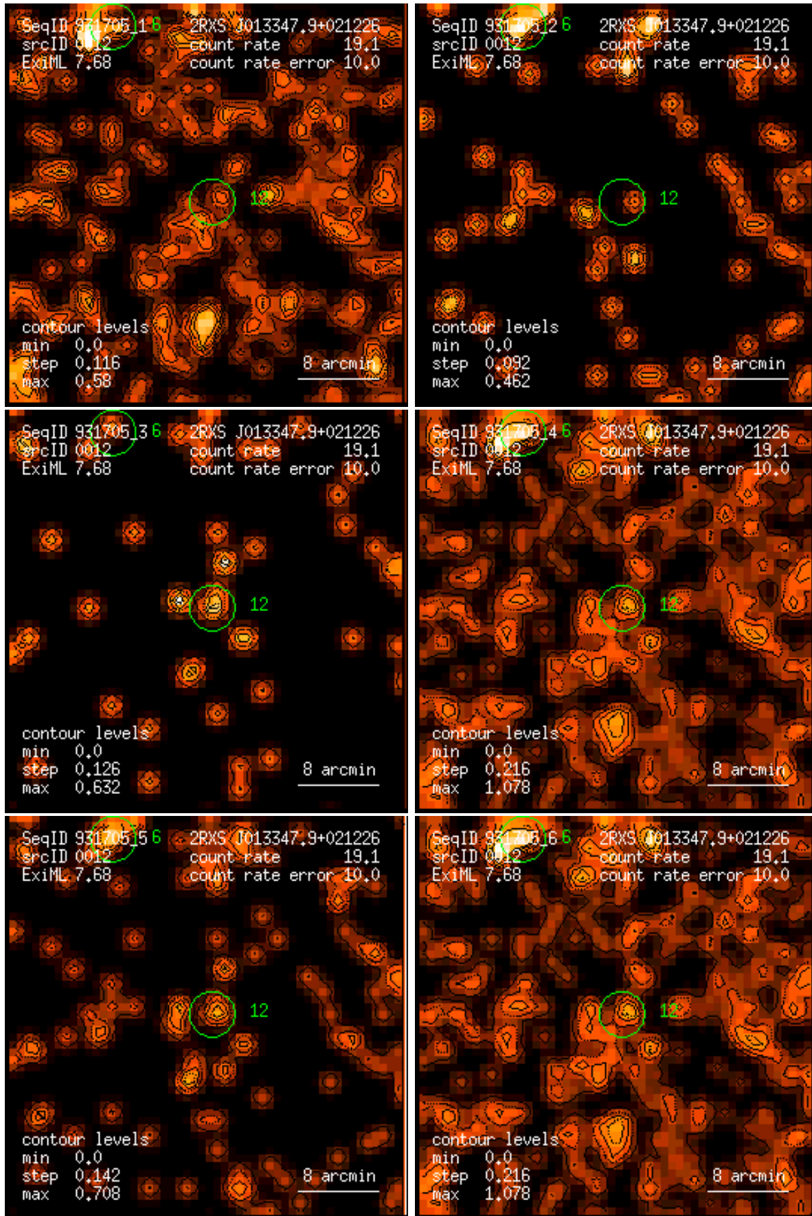
Figure 12: RASS 931705: detection 0012: band rate images, Gaussian filter: (1) PSPC channels 11 – 41, (2) 52 – 90, (3) 91 – 201, (4) 11 – 235, (5) 52 – 201, (6) 11 – 201. Broad band rates in counts/ks. Band rate contour levels in counts/ks/arcmin 2 .
