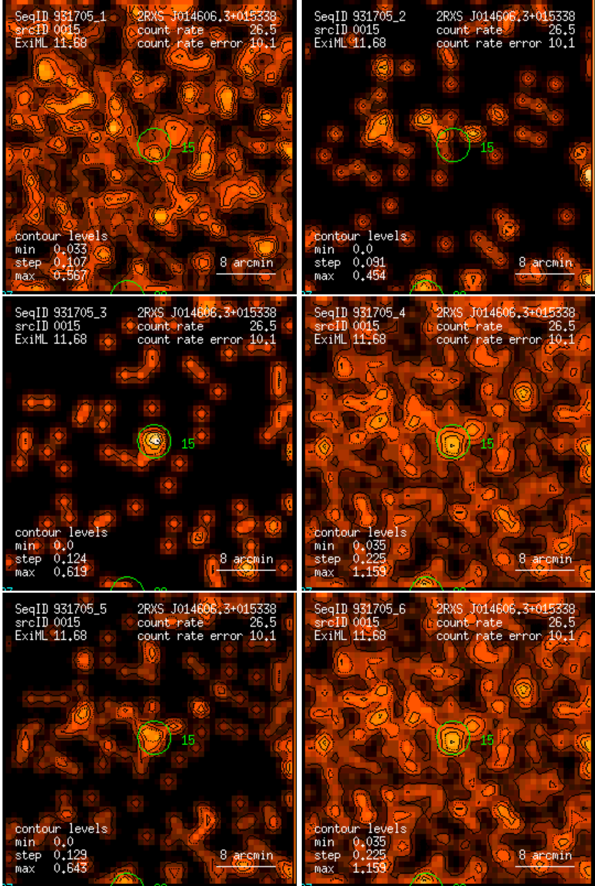
Figure 15: RASS 931705: detection 0015: band rate images, Gaussian filter: (1) PSPC channels 11 – 41, (2) 52 – 90, (3) 91 – 201, (4) 11 – 235, (5) 52 – 201, (6) 11 – 201. Broad band rates in counts/ks. Band rate contour levels in counts/ks/arcmin 2 .
