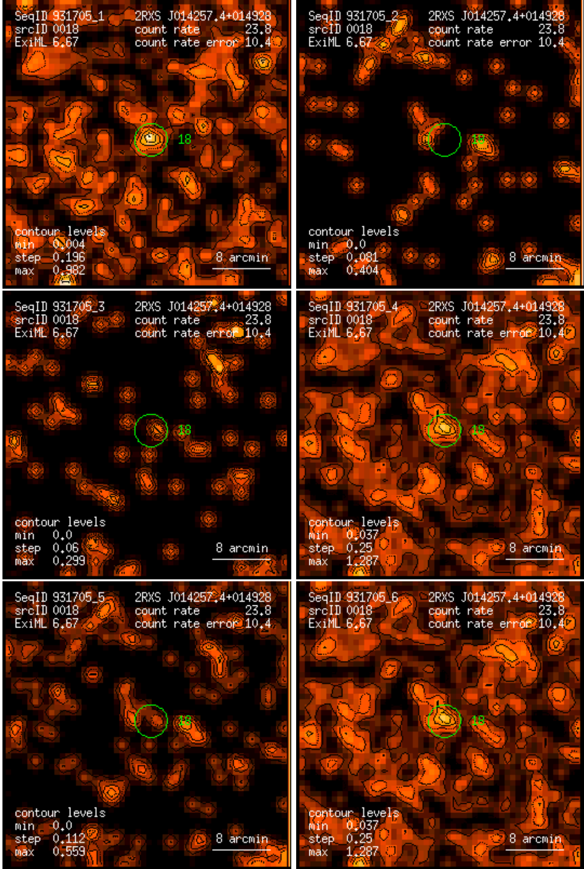
Figure 18: RASS 931705: detection 0018: band rate images, Gaussian filter: (1) PSPC channels 11 – 41, (2) 52 – 90, (3) 91 – 201, (4) 11 – 235, (5) 52 – 201, (6) 11 – 201. Broad band rates in counts/ks. Band rate contour levels in counts/ks/arcmin 2 .
