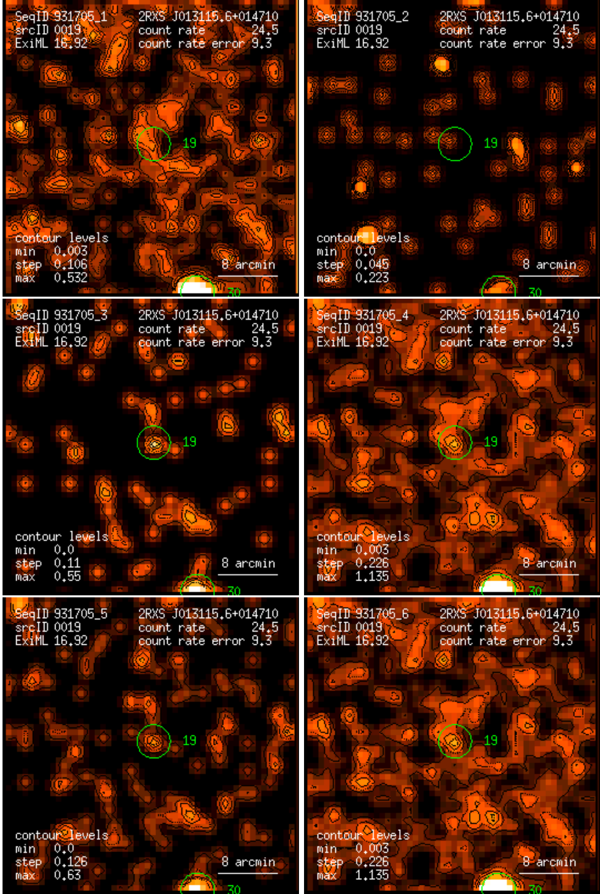
Figure 19: RASS 931705: detection 0019: band rate images, Gaussian filter: (1) PSPC channels 11 – 41, (2) 52 – 90, (3) 91 – 201, (4) 11 – 235, (5) 52 – 201, (6) 11 – 201. Broad band rates in counts/ks. Band rate contour levels in counts/ks/arcmin 2 .
