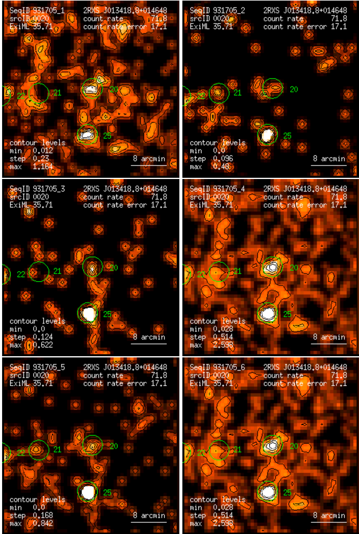
Figure 20: RASS 931705: detection 0020: band rate images, Gaussian filter: (1) PSPC channels 11 – 41, (2) 52 – 90, (3) 91 – 201, (4) 11 – 235, (5) 52 – 201, (6) 11 – 201. Broad band rates in counts/ks. Band rate contour levels in counts/ks/arcmin 2 .
