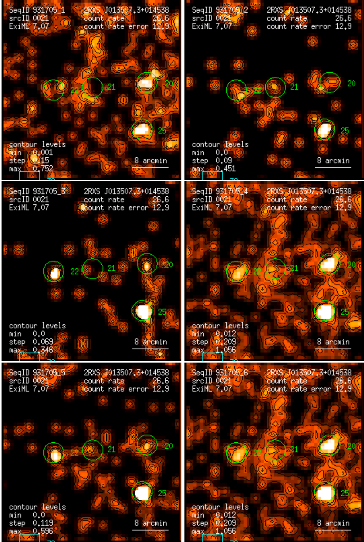
Figure 21: RASS 931705: detection 0021: band rate images, Gaussian filter: (1) PSPC channels 11 – 41, (2) 52 – 90, (3) 91 – 201, (4) 11 – 235, (5) 52 – 201, (6) 11 – 201. Broad band rates in counts/ks. Band rate contour levels in counts/ks/arcmin 2 .
