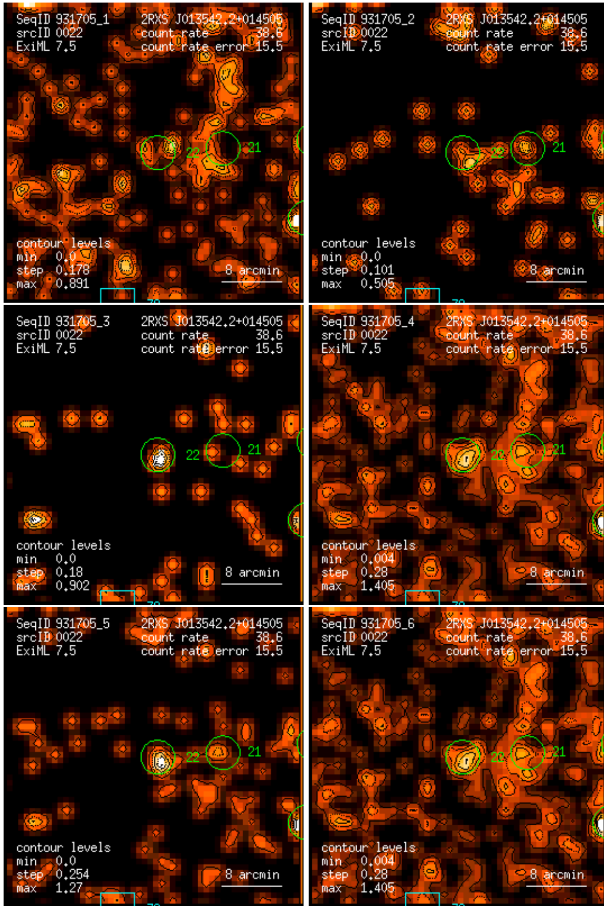
Figure 22: RASS 931705: detection 0022: band rate images, Gaussian filter: (1) PSPC channels 11 – 41, (2) 52 – 90, (3) 91 – 201, (4) 11 – 235, (5) 52 – 201, (6) 11 – 201. Broad band rates in counts/ks. Band rate contour levels in counts/ks/arcmin 2 .
