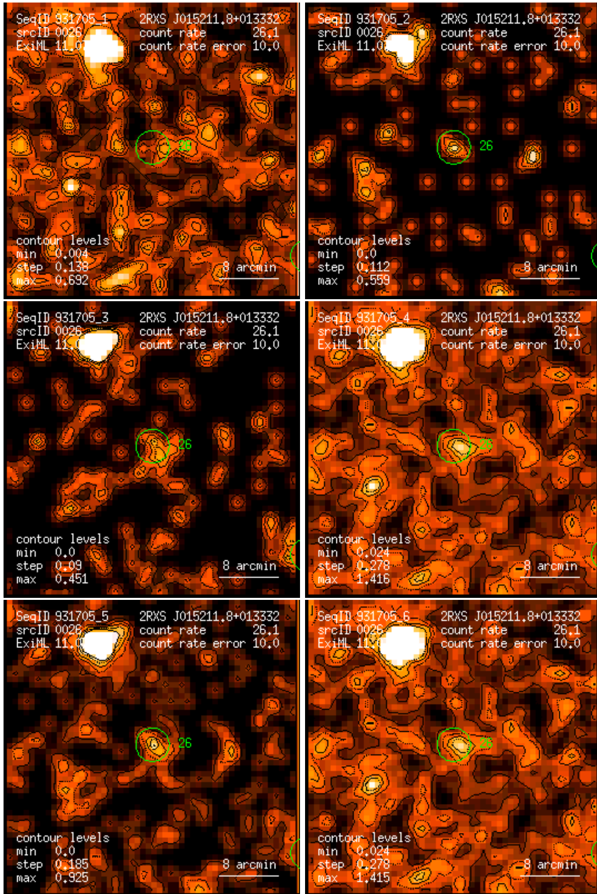
Figure 26: RASS 931705: detection 0026: band rate images, Gaussian filter: (1) PSPC channels 11 – 41, (2) 52 – 90, (3) 91 – 201, (4) 11 – 235, (5) 52 – 201, (6) 11 – 201. Broad band rates in counts/ks. Band rate contour levels in counts/ks/arcmin 2 .
