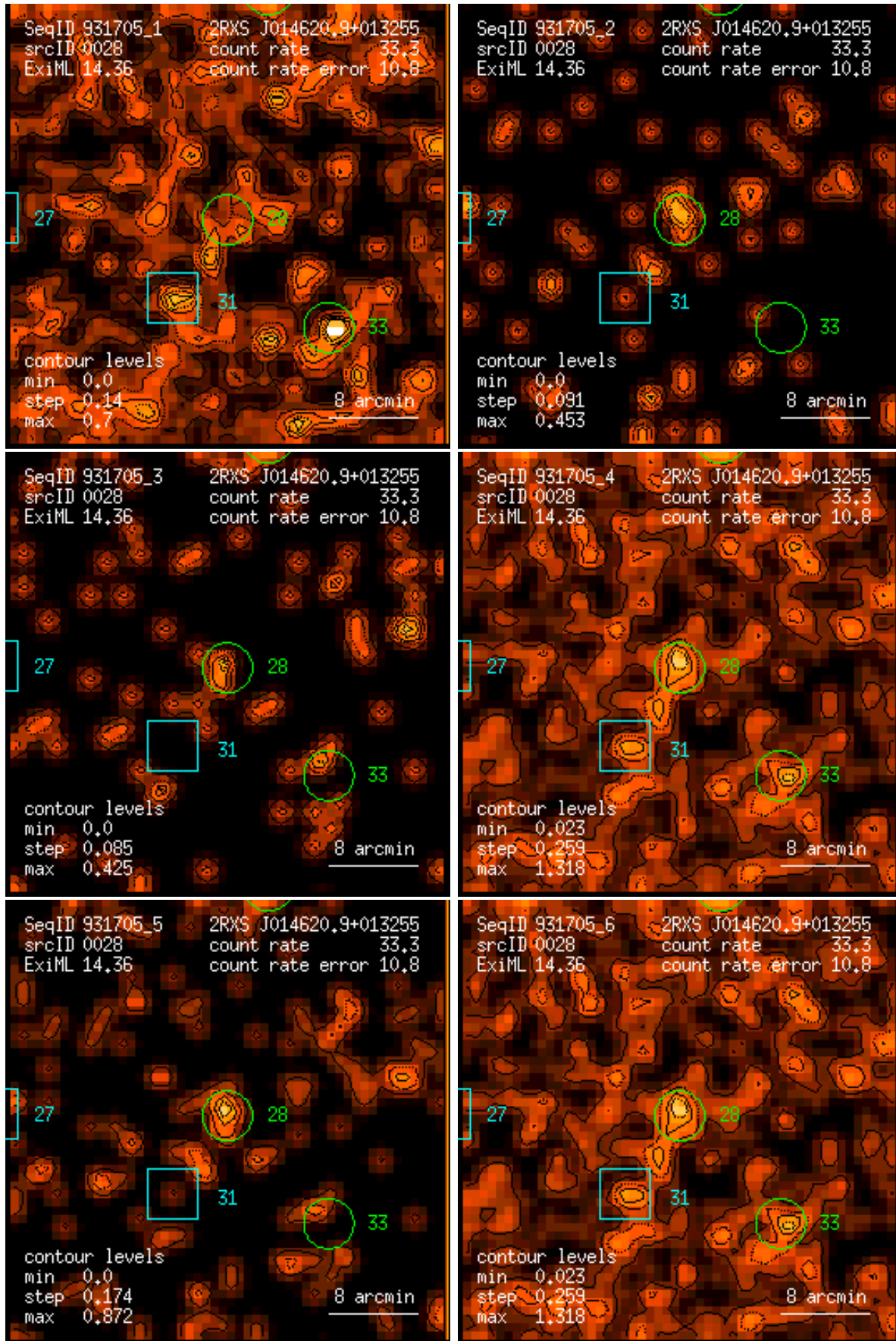
Figure 28: RASS 931705: detection 0028: band rate images, Gaussian filter: (1) PSPC channels 11 – 41, (2) 52 – 90, (3) 91 – 201, (4) 11 – 235, (5) 52 – 201, (6) 11 – 201. Broad band rates in counts/ks. Band rate contour levels in counts/ks/arcmin 2 .
