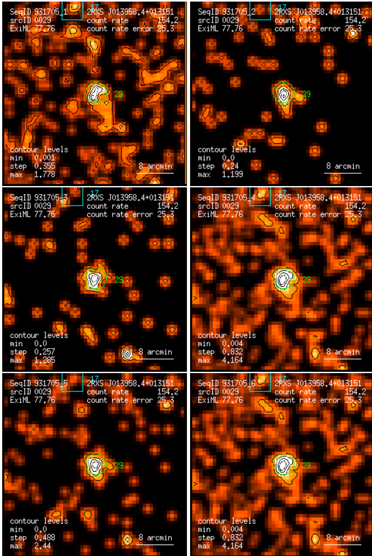
Figure 29: RASS 931705: detection 0029: band rate images, Gaussian filter: (1) PSPC channels 11 – 41, (2) 52 – 90, (3) 91 – 201, (4) 11 – 235, (5) 52 – 201, (6) 11 – 201. Broad band rates in counts/ks. Band rate contour levels in counts/ks/arcmin 2 .
