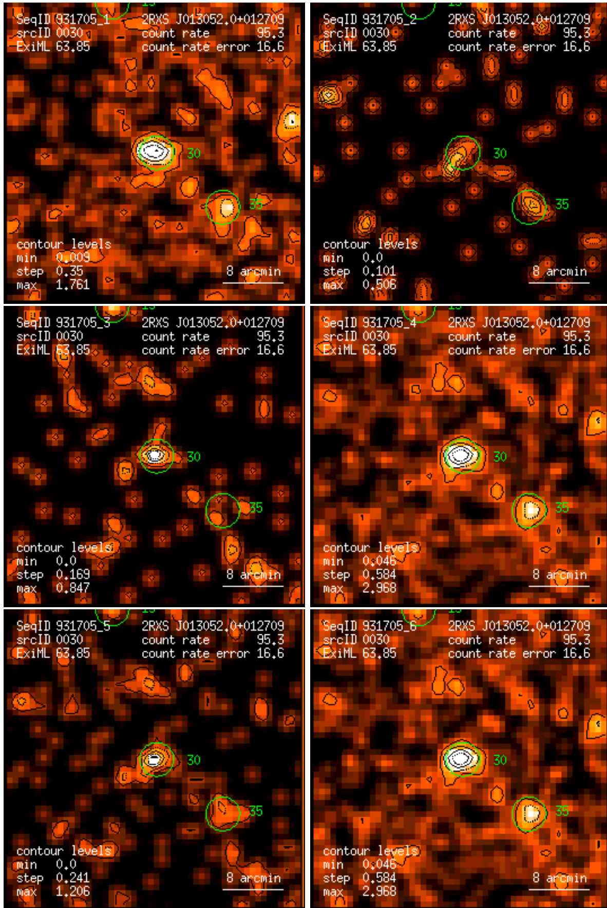
Figure 30: RASS 931705: detection 0030: band rate images, Gaussian filter: (1) PSPC channels 11 – 41, (2) 52 – 90, (3) 91 – 201, (4) 11 – 235, (5) 52 – 201, (6) 11 – 201. Broad band rates in counts/ks. Band rate contour levels in counts/ks/arcmin 2 .
