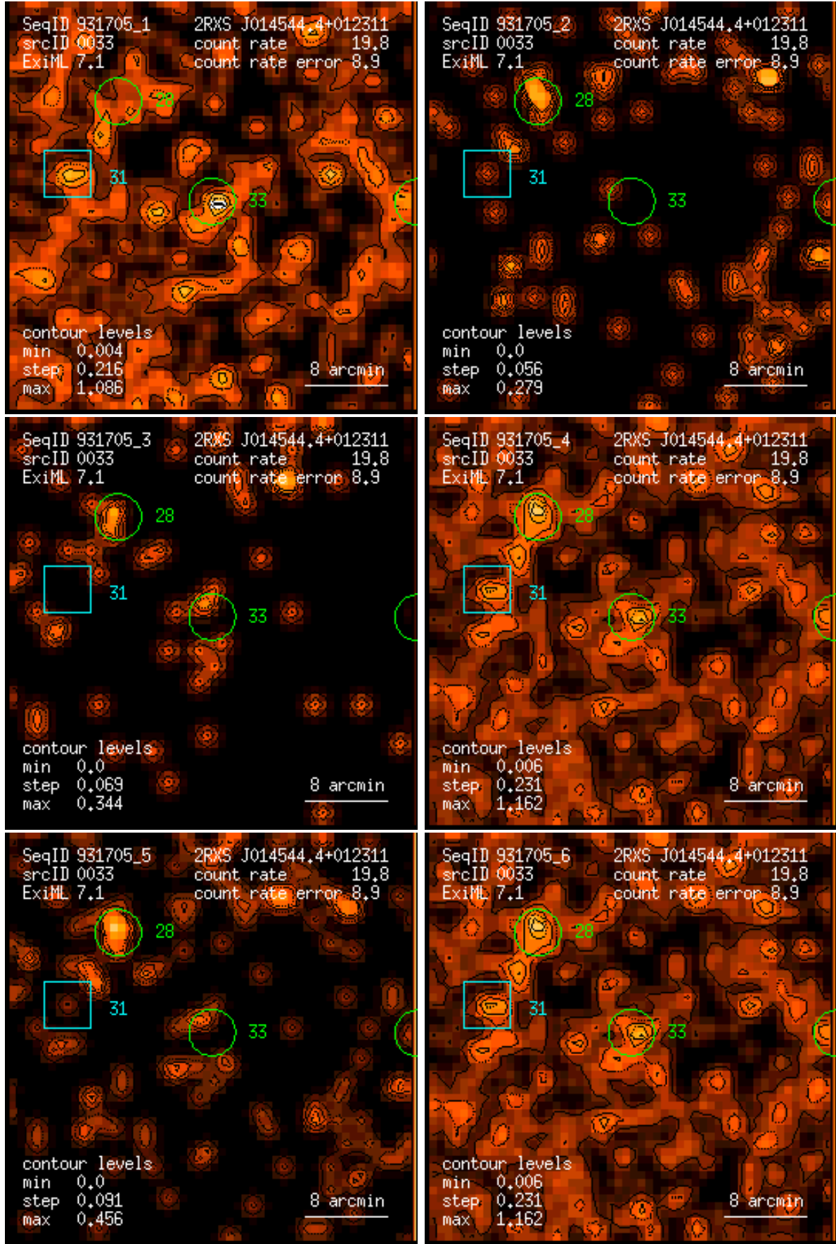
Figure 33: RASS 931705: detection 0033: band rate images, Gaussian filter: (1) PSPC channels 11 – 41, (2) 52 – 90, (3) 91 – 201, (4) 11 – 235, (5) 52 – 201, (6) 11 – 201. Broad band rates in counts/ks. Band rate contour levels in counts/ks/arcmin 2 .
