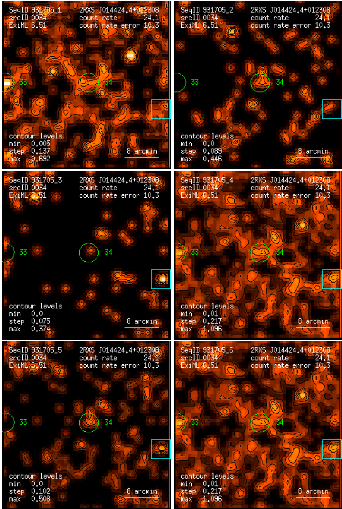
Figure 34: RASS 931705: detection 0034: band rate images, Gaussian filter: (1) PSPC channels 11 – 41, (2) 52 – 90, (3) 91 – 201, (4) 11 – 235, (5) 52 – 201, (6) 11 – 201. Broad band rates in counts/ks. Band rate contour levels in counts/ks/arcmin 2 .
