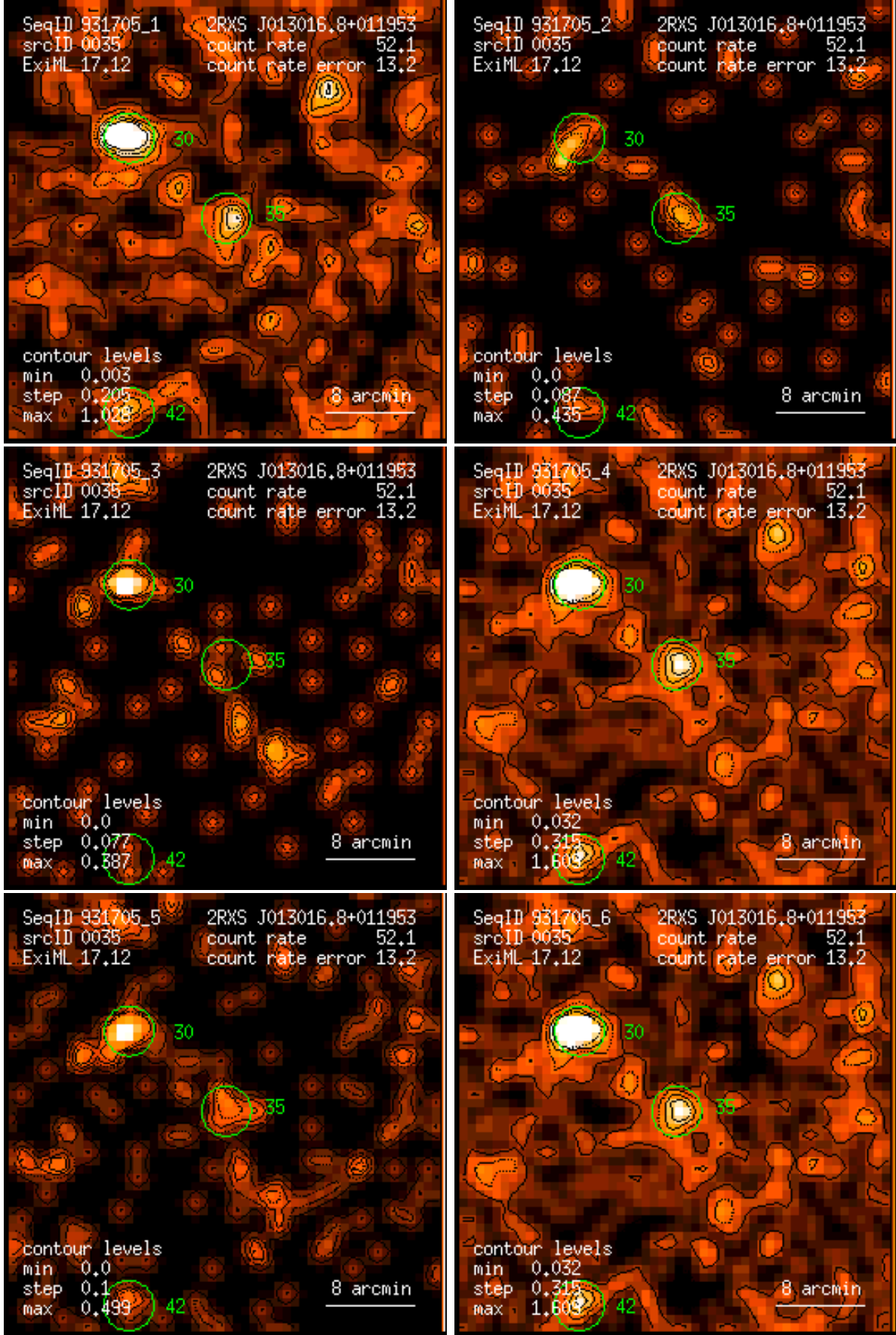
Figure 35: RASS 931705: detection 0035: band rate images, Gaussian filter: (1) PSPC channels 11 – 41, (2) 52 – 90, (3) 91 – 201, (4) 11 – 235, (5) 52 – 201, (6) 11 – 201. Broad band rates in counts/ks. Band rate contour levels in counts/ks/arcmin 2 .
