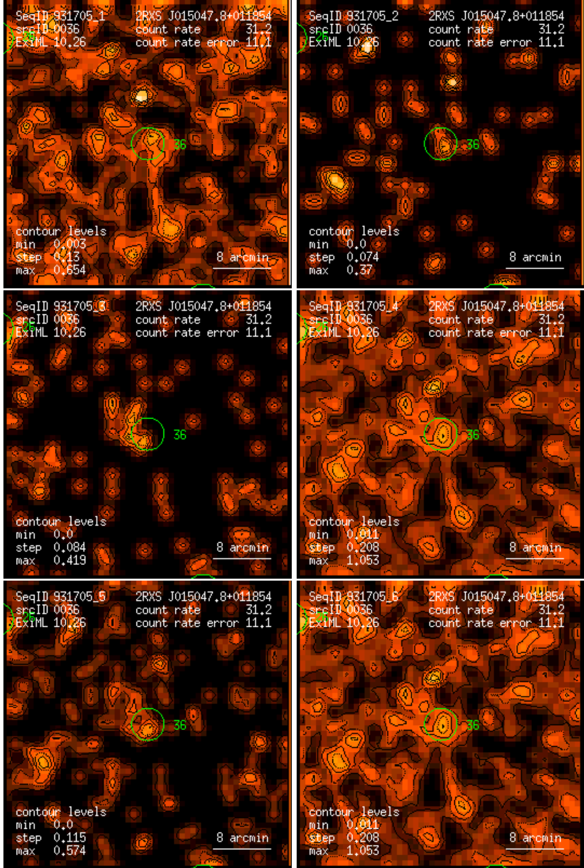
Figure 36: RASS 931705: detection 0036: band rate images, Gaussian filter: (1) PSPC channels 11 – 41, (2) 52 – 90, (3) 91 – 201, (4) 11 – 235, (5) 52 – 201, (6) 11 – 201. Broad band rates in counts/ks. Band rate contour levels in counts/ks/arcmin 2 .
