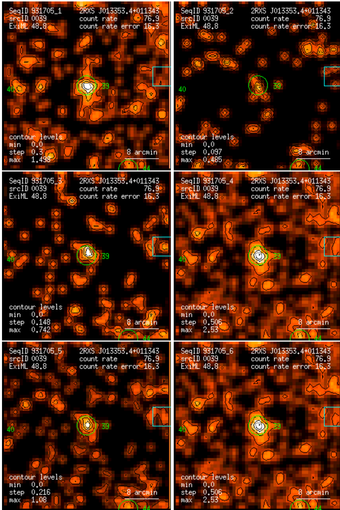
Figure 39: RASS 931705: detection 0039: band rate images, Gaussian filter: (1) PSPPC channels 11 – 41, (2) 52 – 90, (3) 91 – 201, (4) 11 – 235, (5) 52 – 201, (6) 11 – 201. Broad band rates in counts/ks. Band rate contour levels in counts/ks/arcmin 2 .
