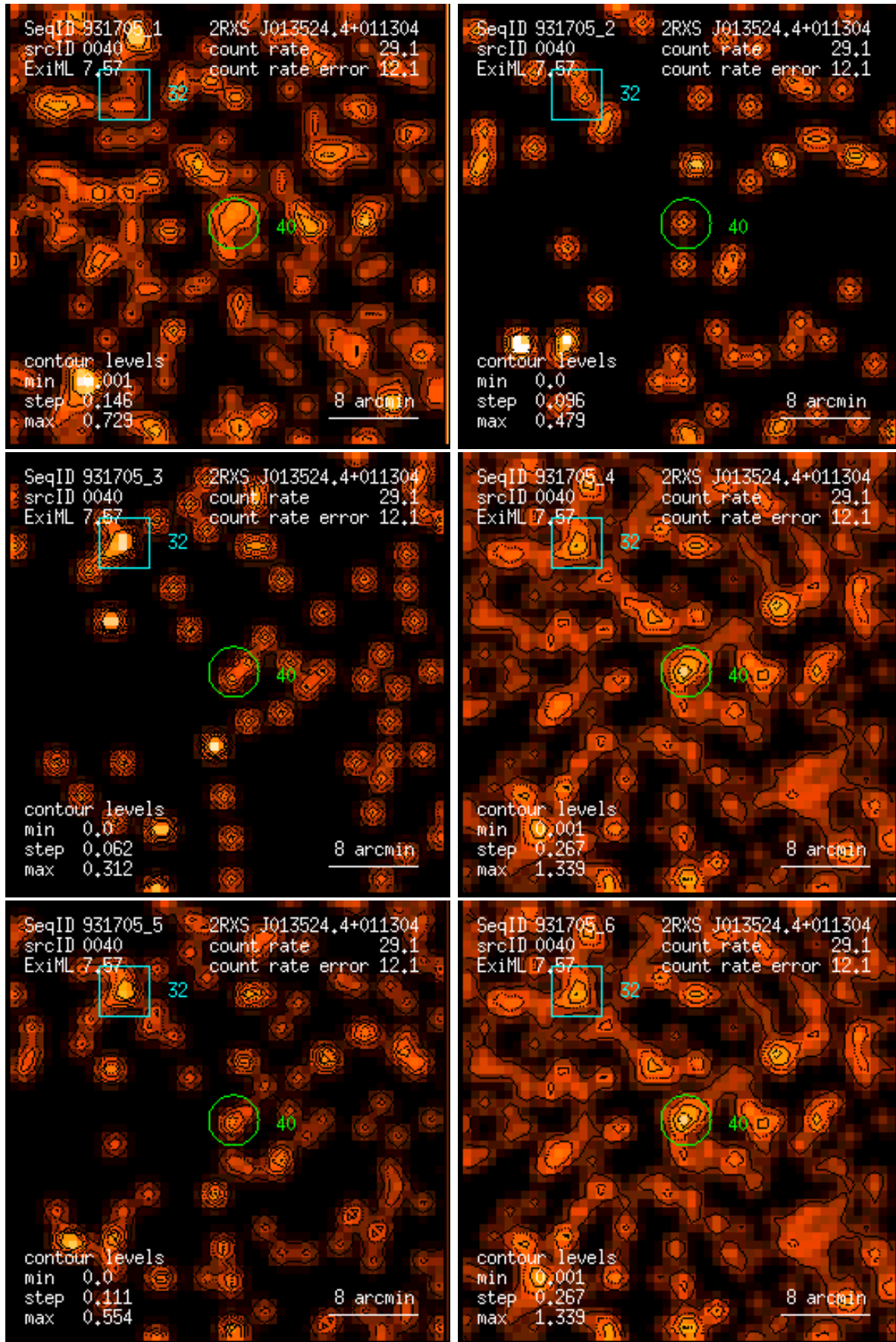
Figure 40: RASS 931705: detection 0040: band rate images, Gaussian filter: (1) PSPC channels 11 – 41, (2) 52 – 90, (3) 91 – 201, (4) 11 – 235, (5) 52 – 201, (6) 11 – 201. Broad band rates in counts/ks. Band rate contour levels in counts/ks/arcmin 2 .
