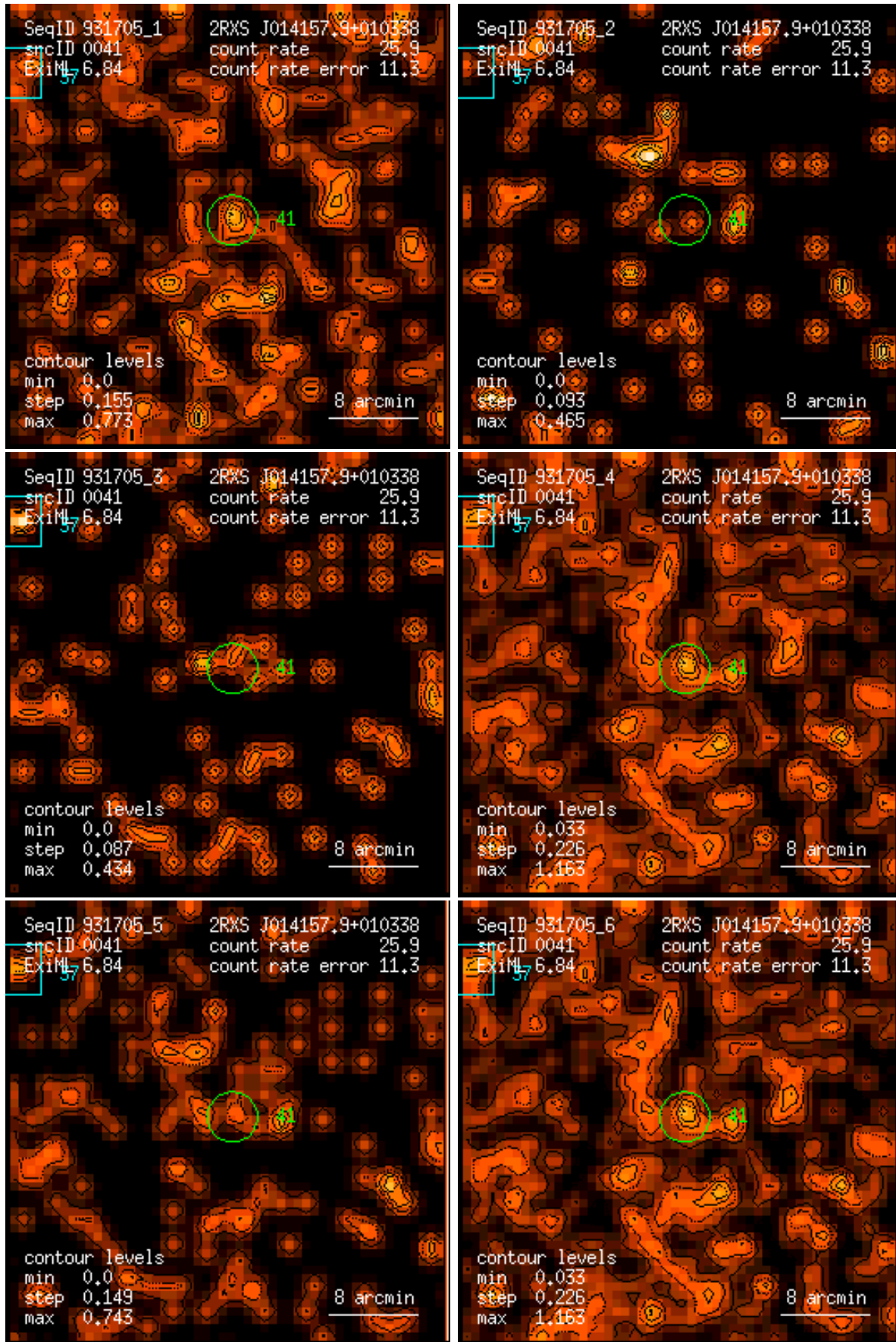
Figure 41: RASS 931705: detection 0041: band rate images, Gaussian filter: (1) PSPC channels 11 – 41, (2) 52 – 90, (3) 91 – 201, (4) 11 – 235, (5) 52 – 201, (6) 11 – 201. Broad band rates in counts/ks. Band rate contour levels in counts/ks/arcmin 2 .
