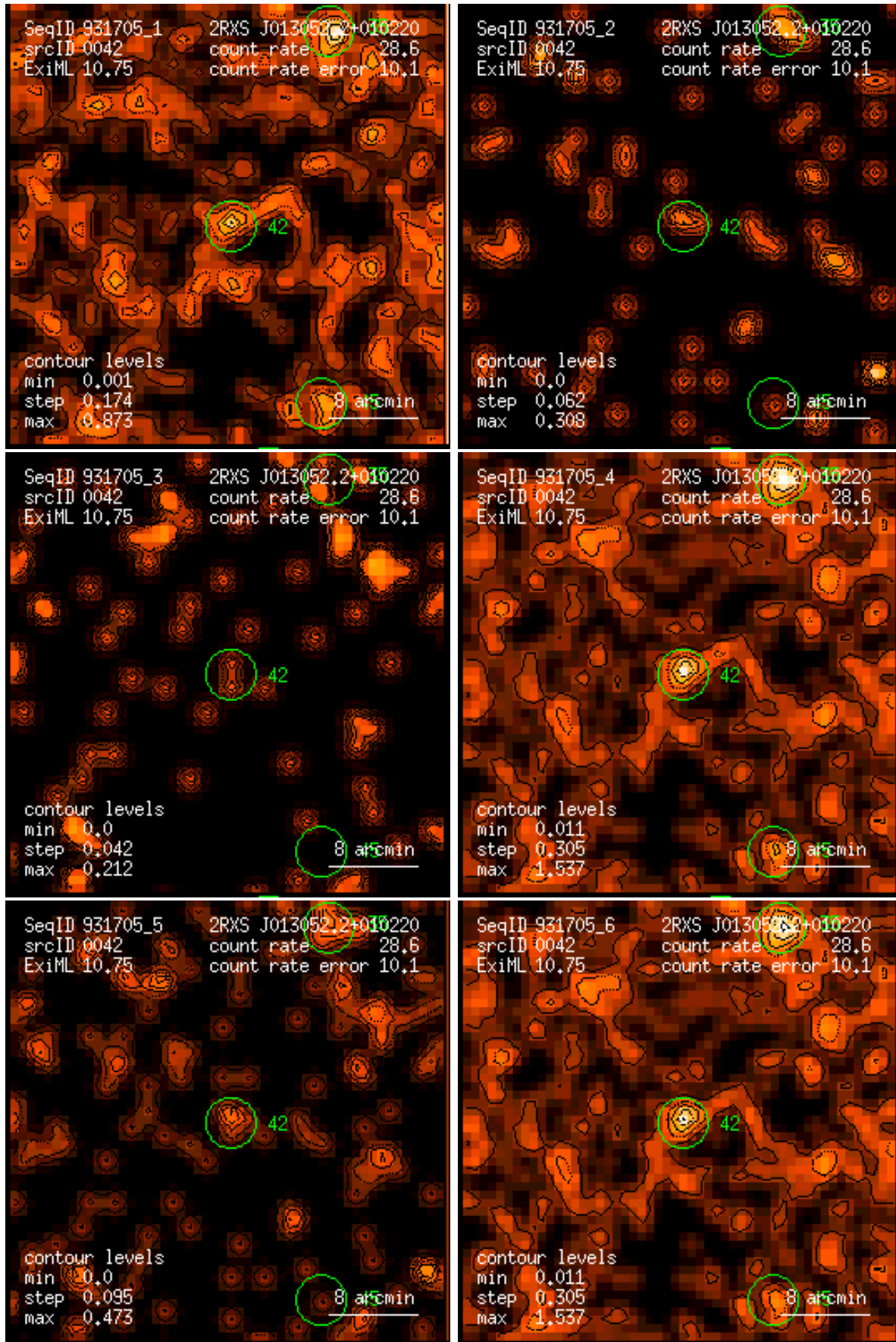
Figure 42: RASS 931705: detection 0042: band rate images, Gaussian filter: (1) PSPC channels 11 – 41, (2) 52 – 90, (3) 91 – 201, (4) 11 – 235, (5) 52 – 201, (6) 11 – 201. Broad band rates in counts/ks. Band rate contour levels in counts/ks/arcmin 2 .
