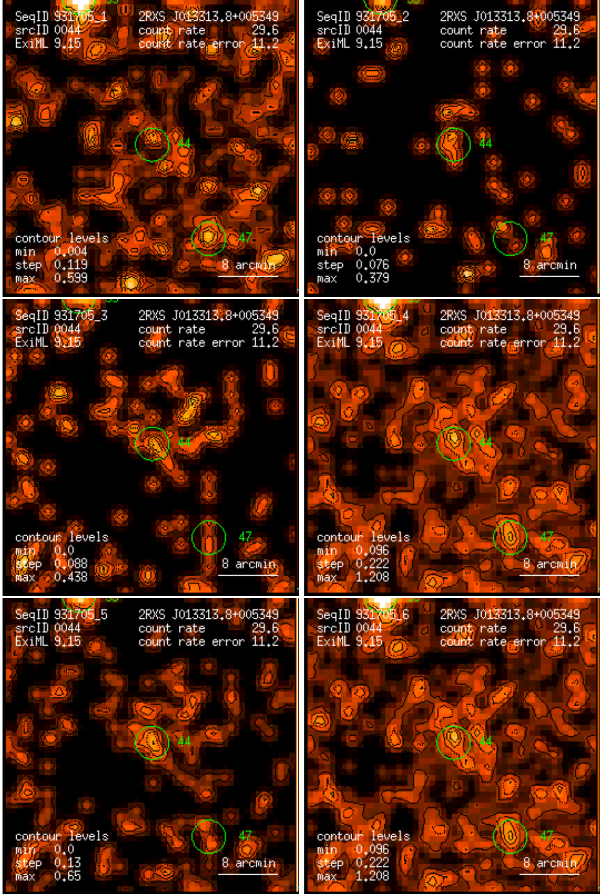
Figure 44: RASS 931705: detection 0044: band rate images, Gaussian filter: (1) PSPC channels 11 – 41, (2) 52 – 90, (3) 91 – 201, (4) 11 – 235, (5) 52 – 201, (6) 11 – 201. Broad band rates in counts/ks. Band rate contour levels in counts/ks/arcmin 2 .
