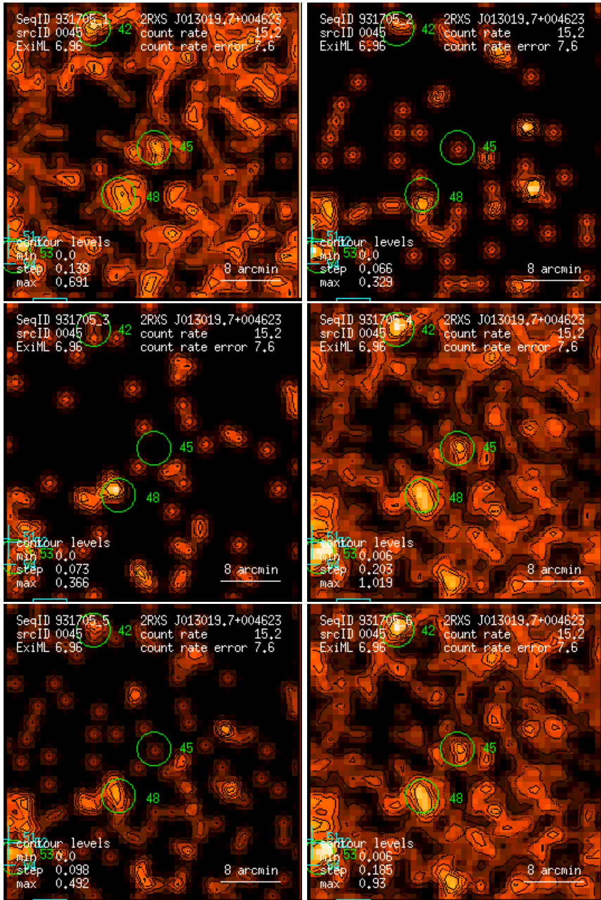
Figure 45: RASS 931705: detection 0045: band rate images, Gaussian filter: (1) PSPC channels 11 – 41, (2) 52 – 90, (3) 91 – 201, (4) 11 – 235, (5) 52 – 201, (6) 11 – 201. Broad band rates in counts/ks. Band rate contour levels in counts/ks/arcmin 2 .
