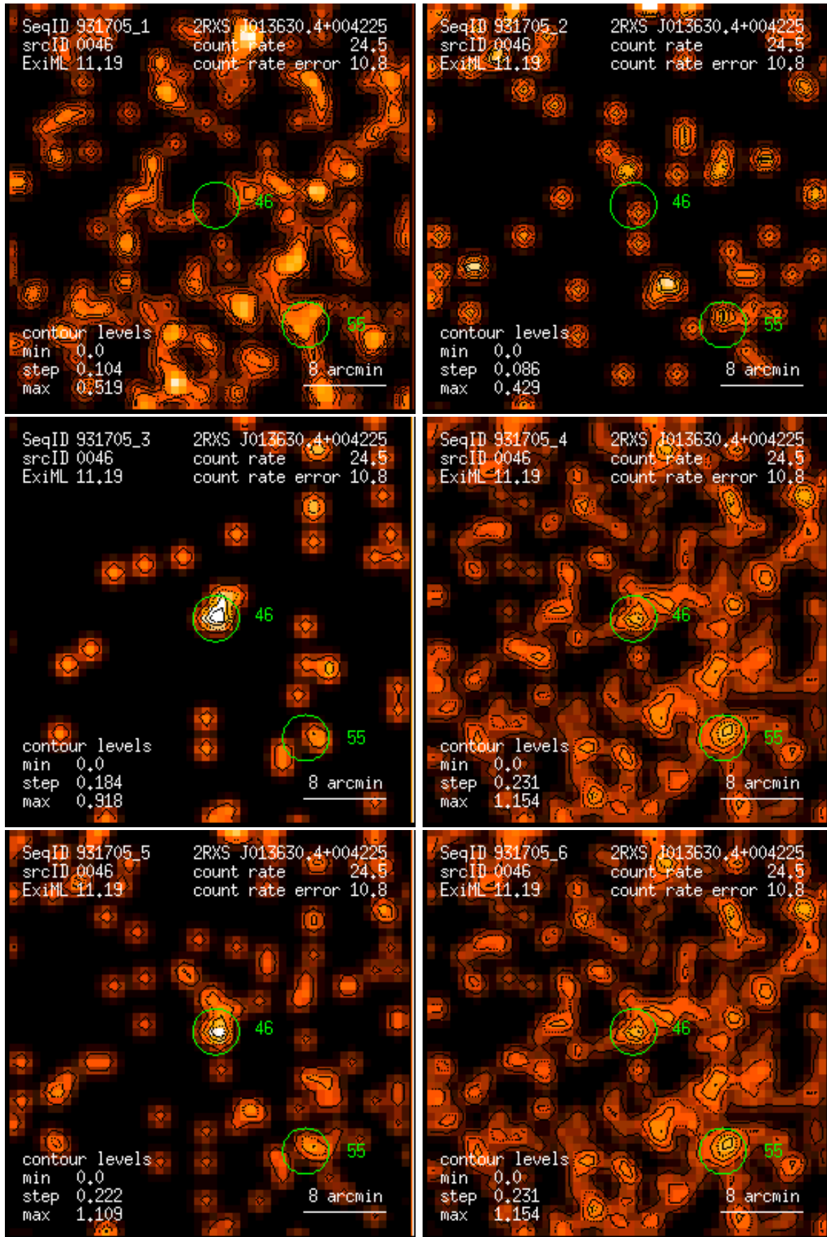
Figure 46: RASS 931705: detection 0046: band rate images, Gaussian filter: (1) PSPC channels 11 – 41, (2) 52 – 90, (3) 91 – 201, (4) 11 – 235, (5) 52 – 201, (6) 11 – 201. Broad band rates in counts/ks. Band rate contour levels in counts/ks/arcmin 2 .
