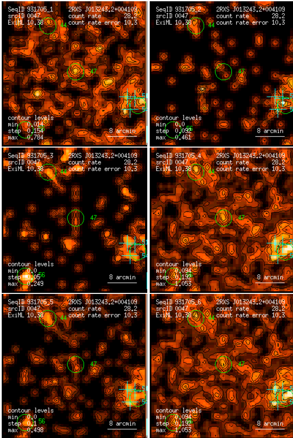
Figure 47: RASS 931705: detection 0047: band rate images, Gaussian filter: (1) PSPC channels 11 – 41, (2) 52 – 90, (3) 91 – 201, (4) 11 – 235, (5) 52 – 201, (6) 11 – 201. Broad band rates in counts/ks. Band rate contour levels in counts/ks/arcmin 2 .
