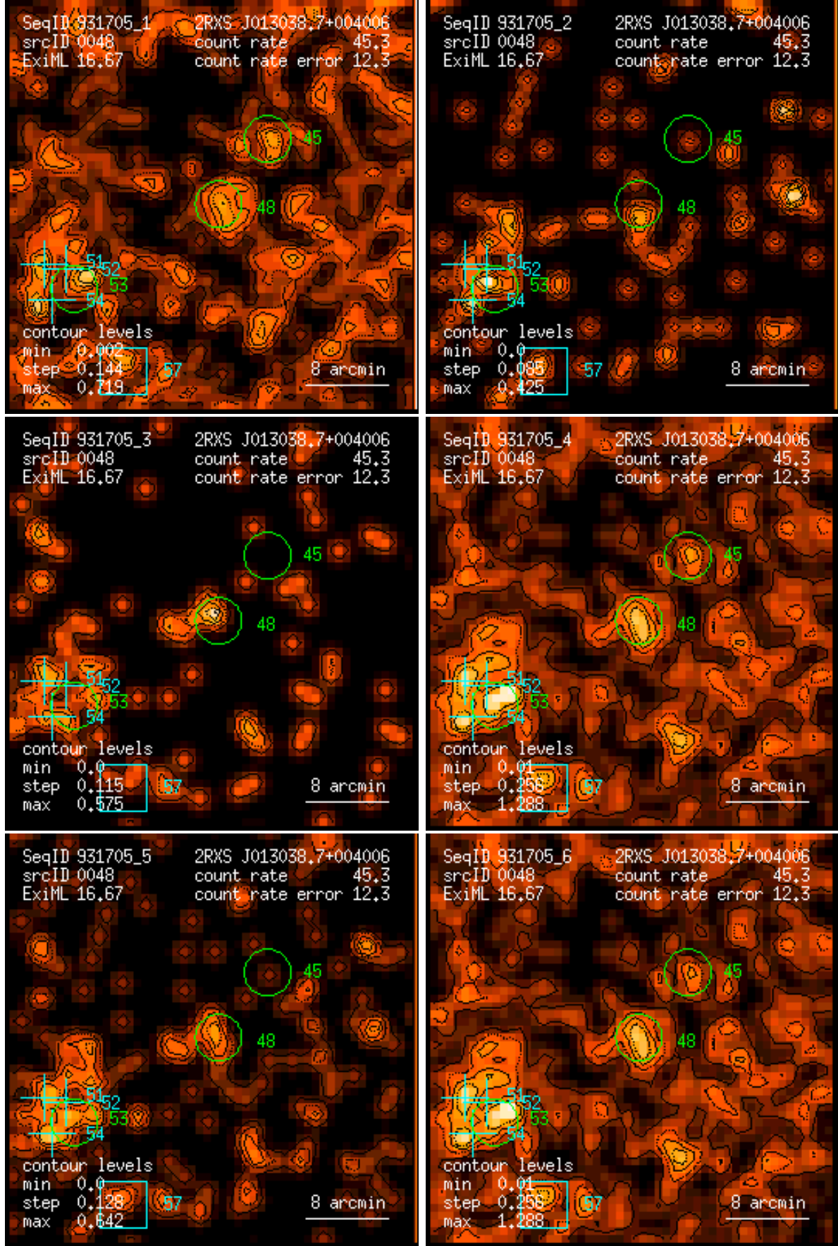
Figure 48: RASS 931705: detection 0048: band rate images, Gaussian filter: (1) PSPC channels 11 – 41, (2) 52 – 90, (3) 91 – 201, (4) 11 – 235, (5) 52 – 201, (6) 11 – 201. Broad band rates in counts/ks. Band rate contour levels in counts/ks/arcmin 2 .
