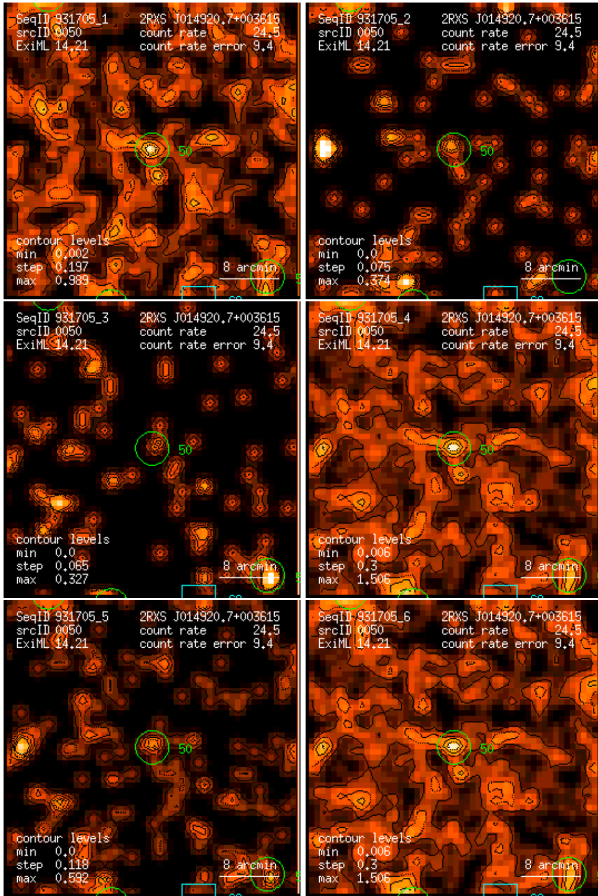
Figure 50: RASS 931705: detection 0050: band rate images, Gaussian filter: (1) PSPC channels 11 – 41, (2) 52 – 90, (3) 91 – 201, (4) 11 – 235, (5) 52 – 201, (6) 11 – 201. Broad band rates in counts/ks. Band rate contour levels in counts/ks/arcmin 2 .
