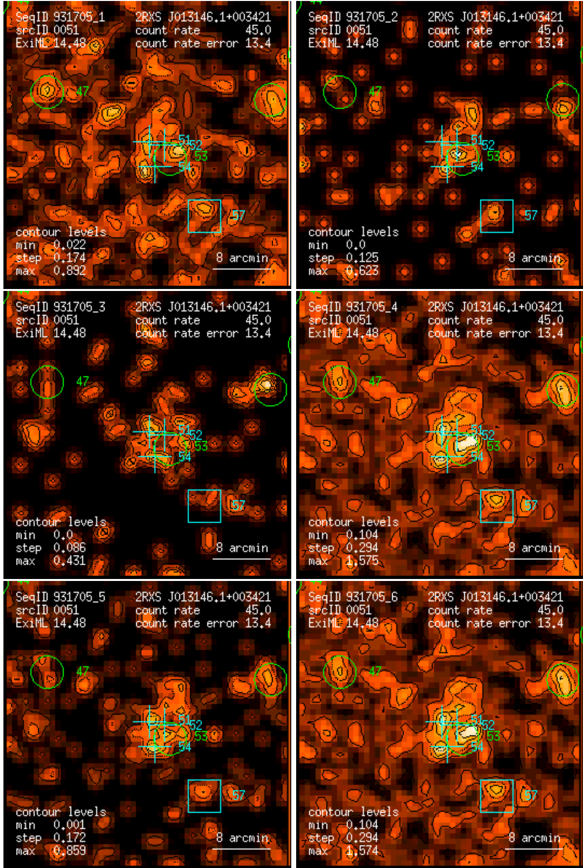
Figure 51: RASS 931705: detection 0051: band rate images, Gaussian filter: (1) PSPC channels 11 – 41, (2) 52 – 90, (3) 91 – 201, (4) 11 – 235, (5) 52 – 201, (6) 11 – 201. Broad band rates in counts/ks. Band rate contour levels in counts/ks/arcmin 2 .
