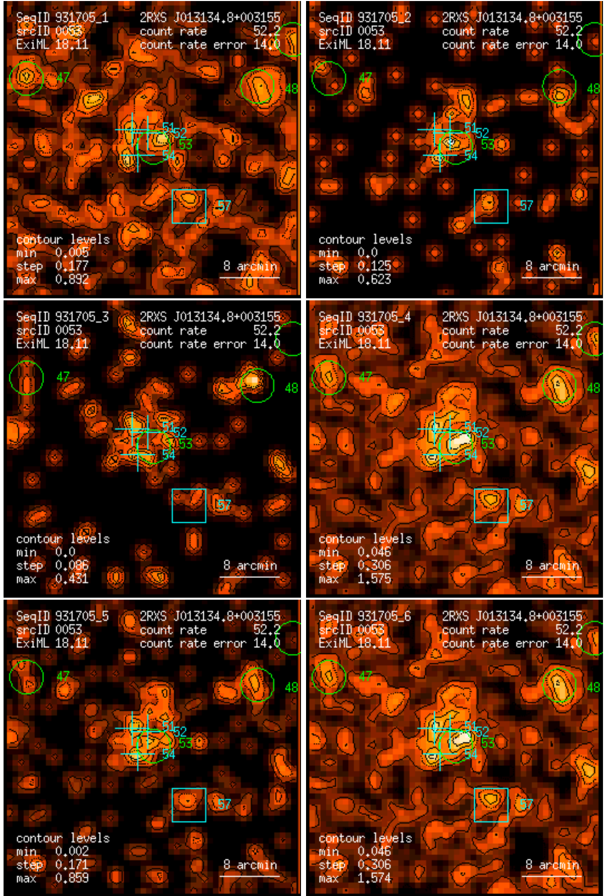
Figure 53: RASS 931705: detection 0053: band rate images, Gaussian filter: (1) PSPC channels 11 – 41, (2) 52 – 90, (3) 91 – 201, (4) 11 – 235, (5) 52 – 201, (6) 11 – 201. Broad band rates in counts/ks. Band rate contour levels in counts/ks/arcmin 2 .
