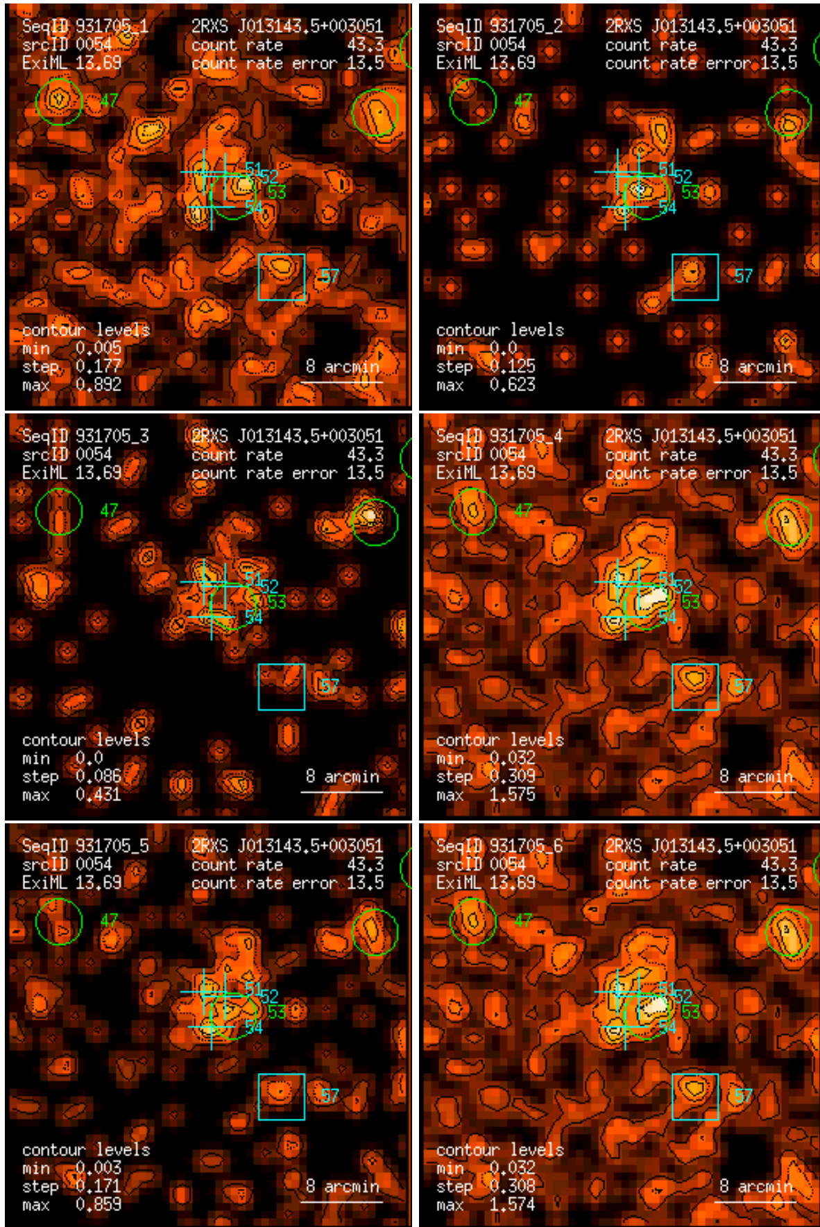
Figure 54: RASS 931705: detection 0054: band rate images, Gaussian filter: (1) PSPC channels 11 – 41, (2) 52 – 90, (3) 91 – 201, (4) 11 – 235, (5) 52 – 201, (6) 11 – 201. Broad band rates in counts/ks. Band rate contour levels in counts/ks/arcmin 2 .
