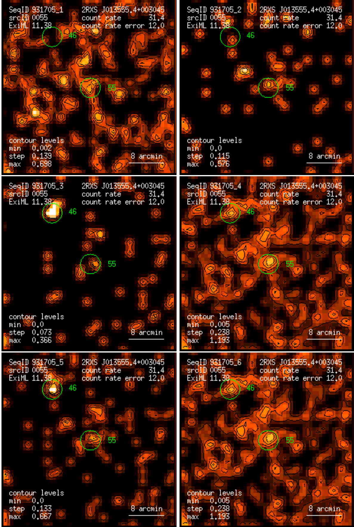
Figure 55: RASS 931705: detection 0055: band rate images, Gaussian filter: (1) PSPC channels 11 – 41, (2) 52 – 90, (3) 91 – 201, (4) 11 – 235, (5) 52 – 201, (6) 11 – 201. Broad band rates in counts/ks. Band rate contour levels in counts/ks/arcmin 2 .
