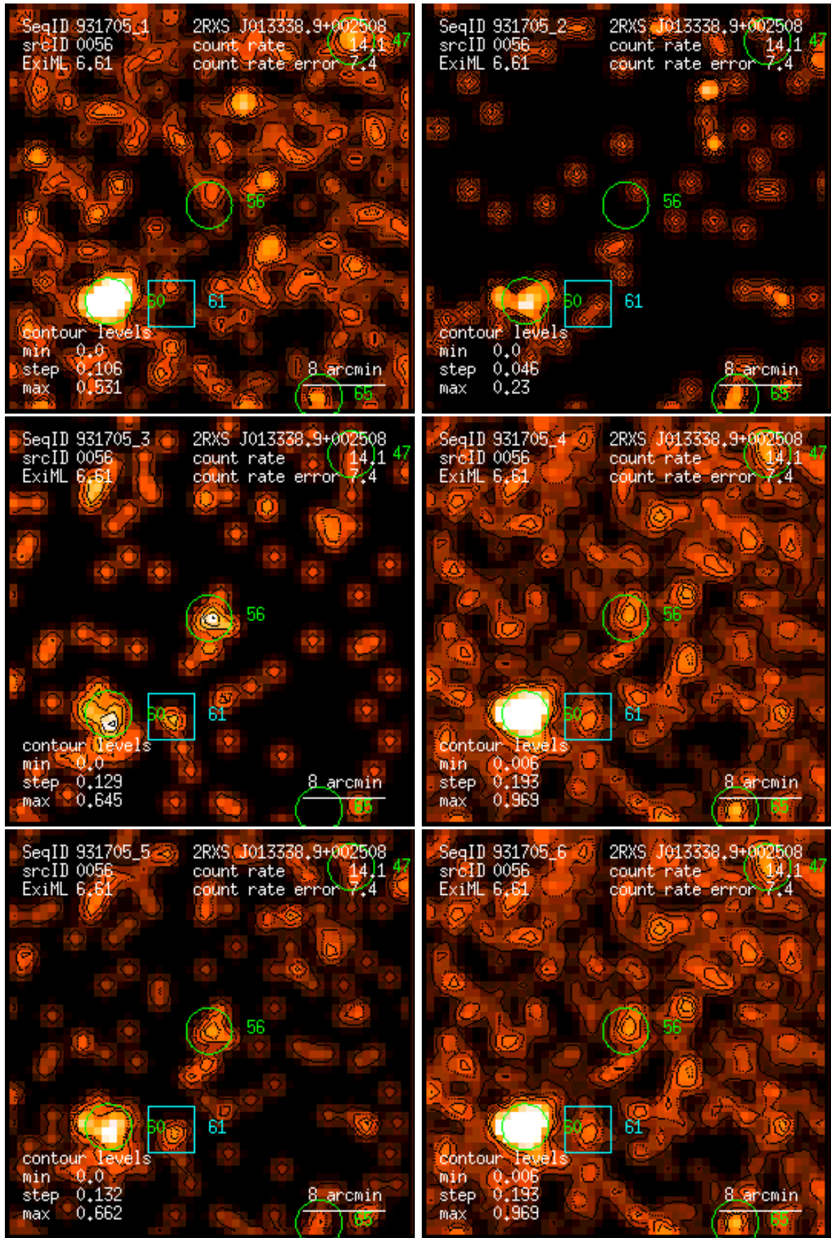
Figure 56: RASS 931705: detection 0056: band rate images, Gaussian filter: (1) PSPC channels 11 – 41, (2) 52 – 90, (3) 91 – 201, (4) 11 – 235, (5) 52 – 201, (6) 11 – 201. Broad band rates in counts/ks. Band rate contour levels in counts/ks/arcmin 2 .
