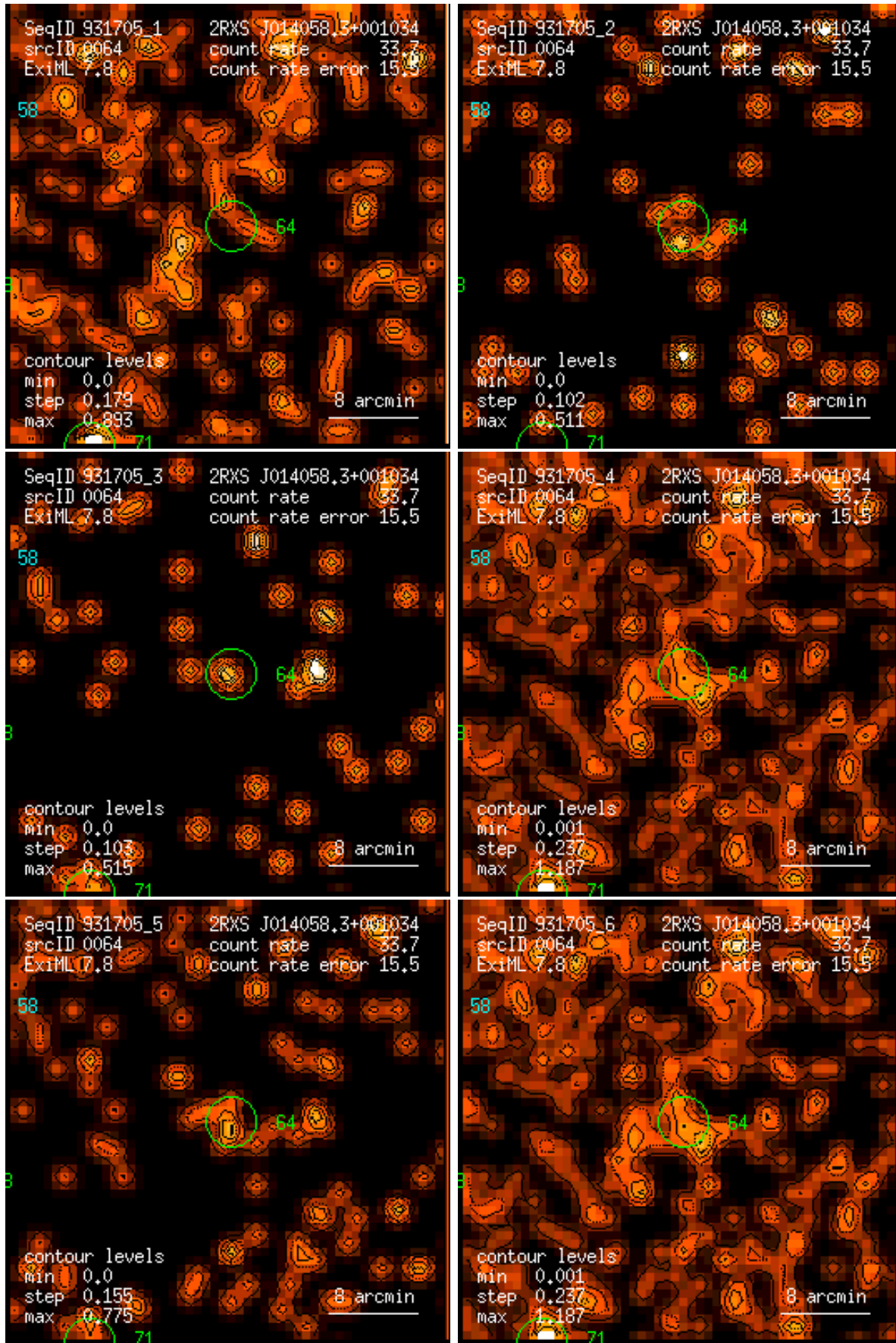
Figure 64: RASS 931705: detection 0064: band rate images, Gaussian filter: (1) PSPC channels 11 – 41, (2) 52 – 90, (3) 91 – 201, (4) 11 – 235, (5) 52 – 201, (6) 11 – 201. Broad band rates in counts/ks. Band rate contour levels in counts/ks/arcmin 2 .
