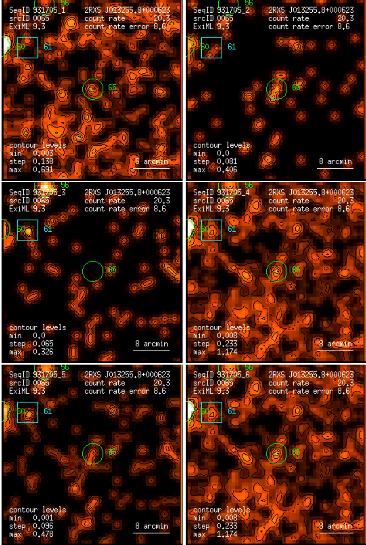
Figure 65: RASS 931705: detection 0065: band rate images, Gaussian filter: (1) PSPC channels 11 – 41, (2) 52 – 90, (3) 91 – 201, (4) 11 – 235, (5) 52 – 201, (6) 11 – 201. Broad band rates in counts/ks. Band rate contour levels in counts/ks/arcmin 2 .
