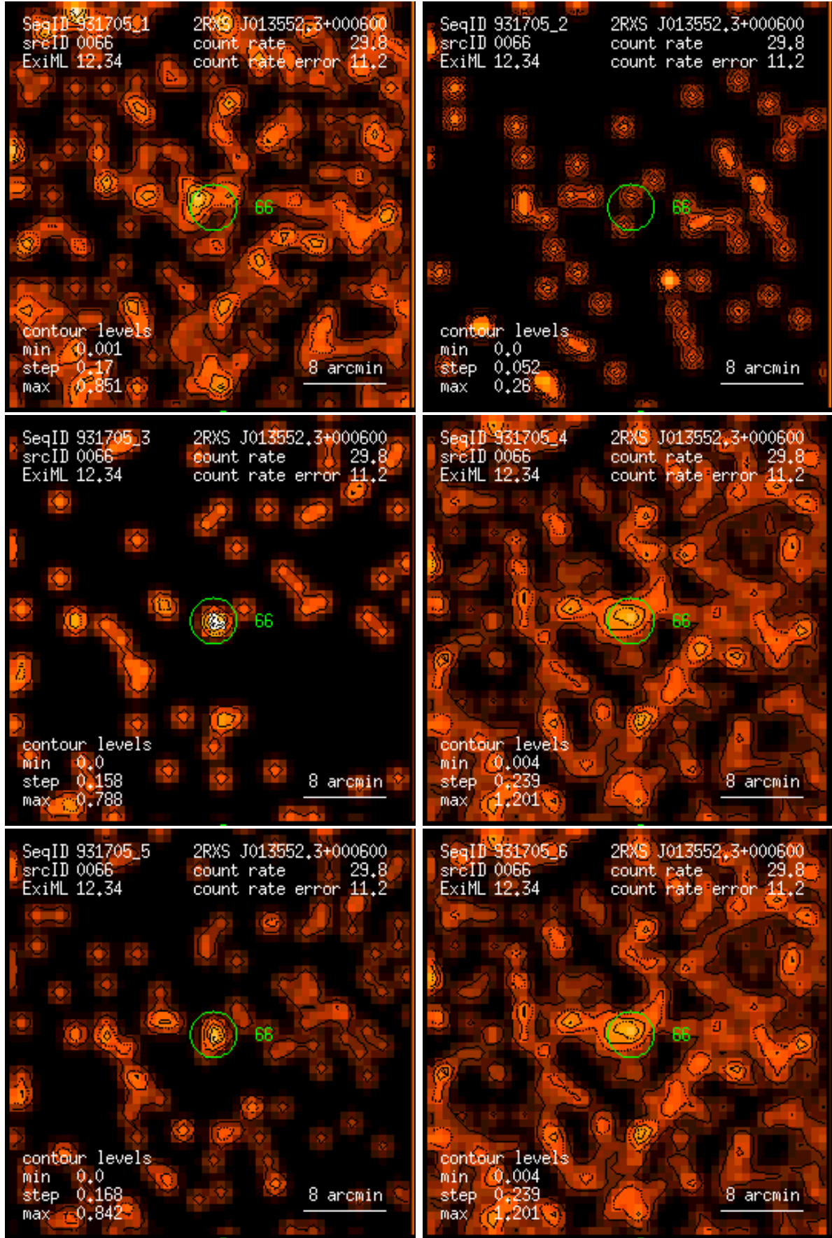
Figure 66: RASS 931705: detection 0066: band rate images, Gaussian filter: (1) PSPC channels 11 – 41, (2) 52 – 90, (3) 91 – 201, (4) 11 – 235, (5) 52 – 201, (6) 11 – 201. Broad band rates in counts/ks. Band rate contour levels in counts/ks/arcmin 2 .
