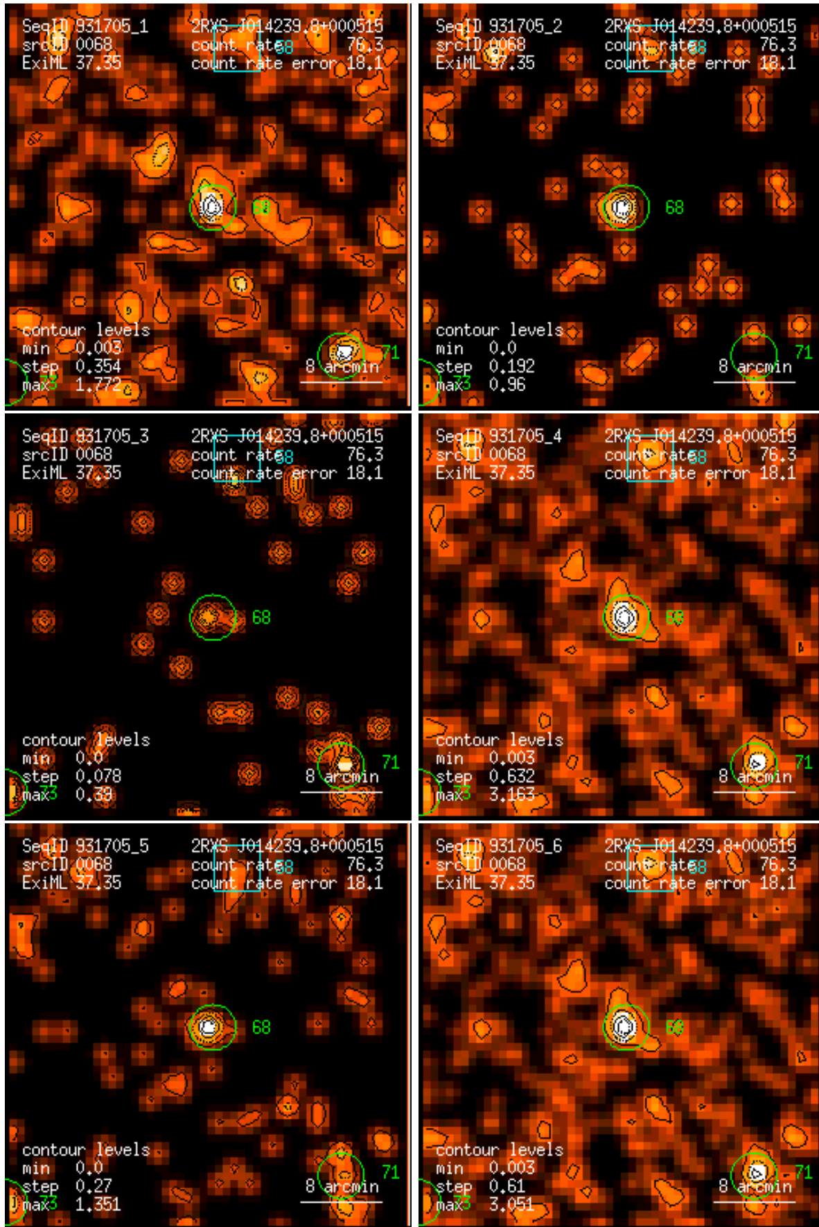
Figure 68: RASS 931705: detection 0068: band rate images, Gaussian filter: (1) PSPC channels 11 – 41, (2) 52 – 90, (3) 91 – 201, (4) 11 – 235, (5) 52 – 201, (6) 11 – 201. Broad band rates in counts/ks. Band rate contour levels in counts/ks/arcmin 2 .
