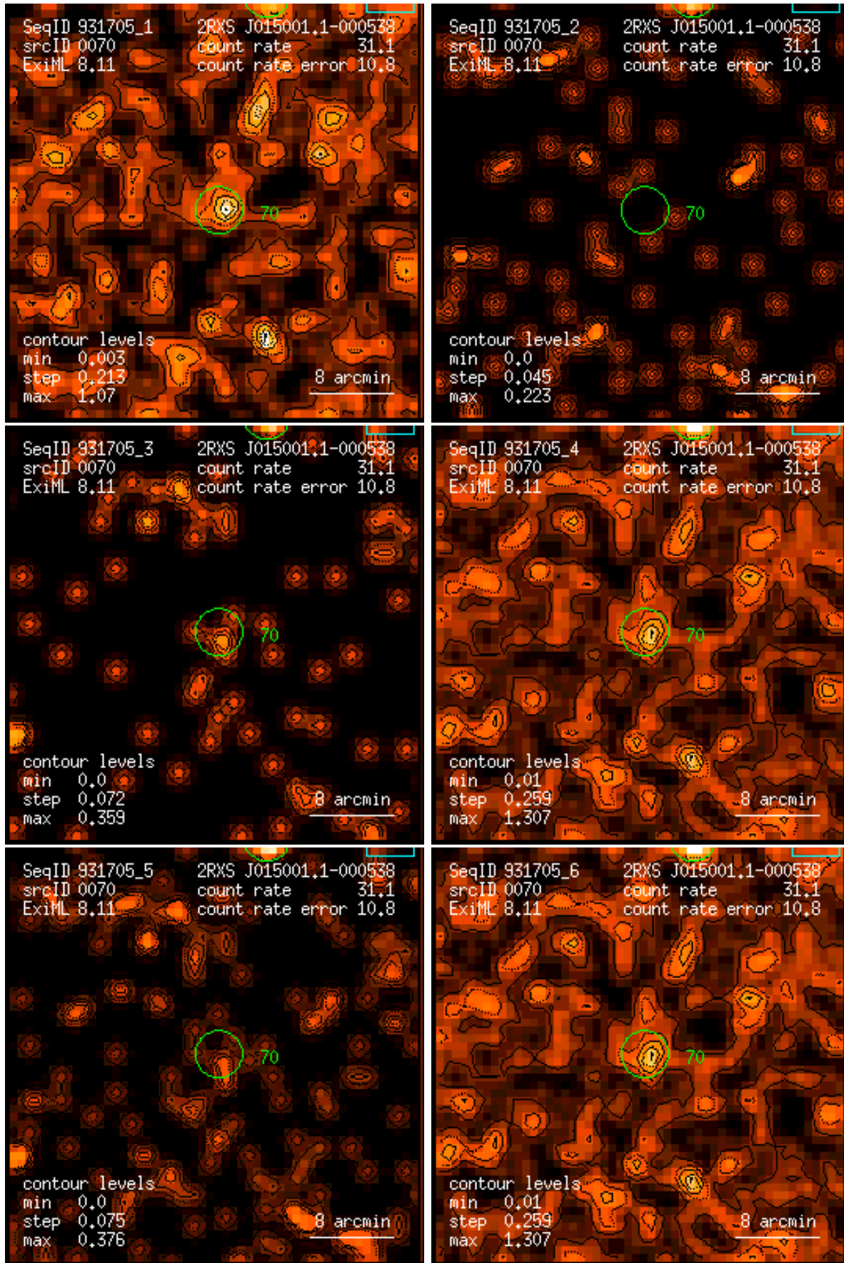
Figure 70: RASS 931705: detection 0070: band rate images, Gaussian filter: (1) PSPC channels 11 – 41, (2) 52 – 90, (3) 91 – 201, (4) 11 – 235, (5) 52 – 201, (6) 11 – 201. Broad band rates in counts/ks. Band rate contour levels in counts/ks/arcmin 2 .
