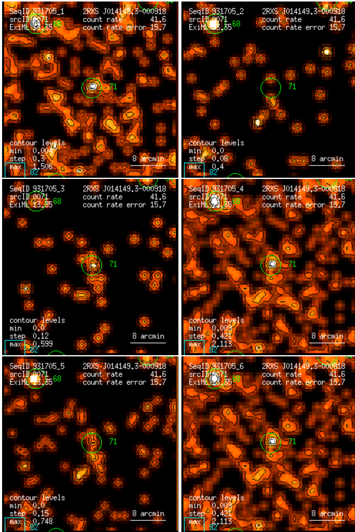
Figure 71: RASS 931705: detection 0071: band rate images, Gaussian filter: (1) PSPC channels 11 – 41, (2) 52 – 90, (3) 91 – 201, (4) 11 – 235, (5) 52 – 201, (6) 11 – 201. Broad band rates in counts/ks. Band rate contour levels in counts/ks/arcmin 2 .
