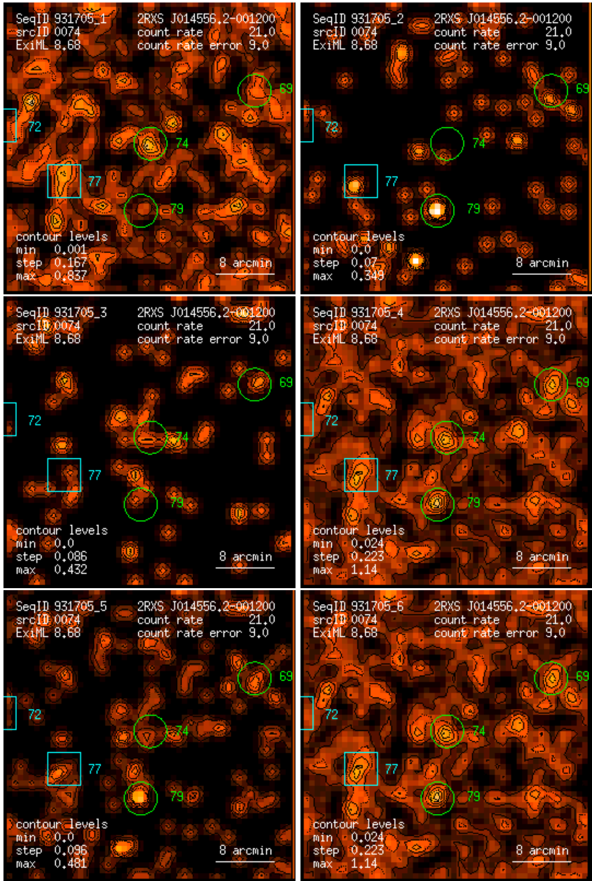
Figure 74: RASS 931705: detection 0074: band rate images, Gaussian filter: (1) PSPC channels 11 – 41, (2) 52 – 90, (3) 91 – 201, (4) 11 – 235, (5) 52 – 201, (6) 11 – 201. Broad band rates in counts/ks. Band rate contour levels in counts/ks/arcmin 2 .
