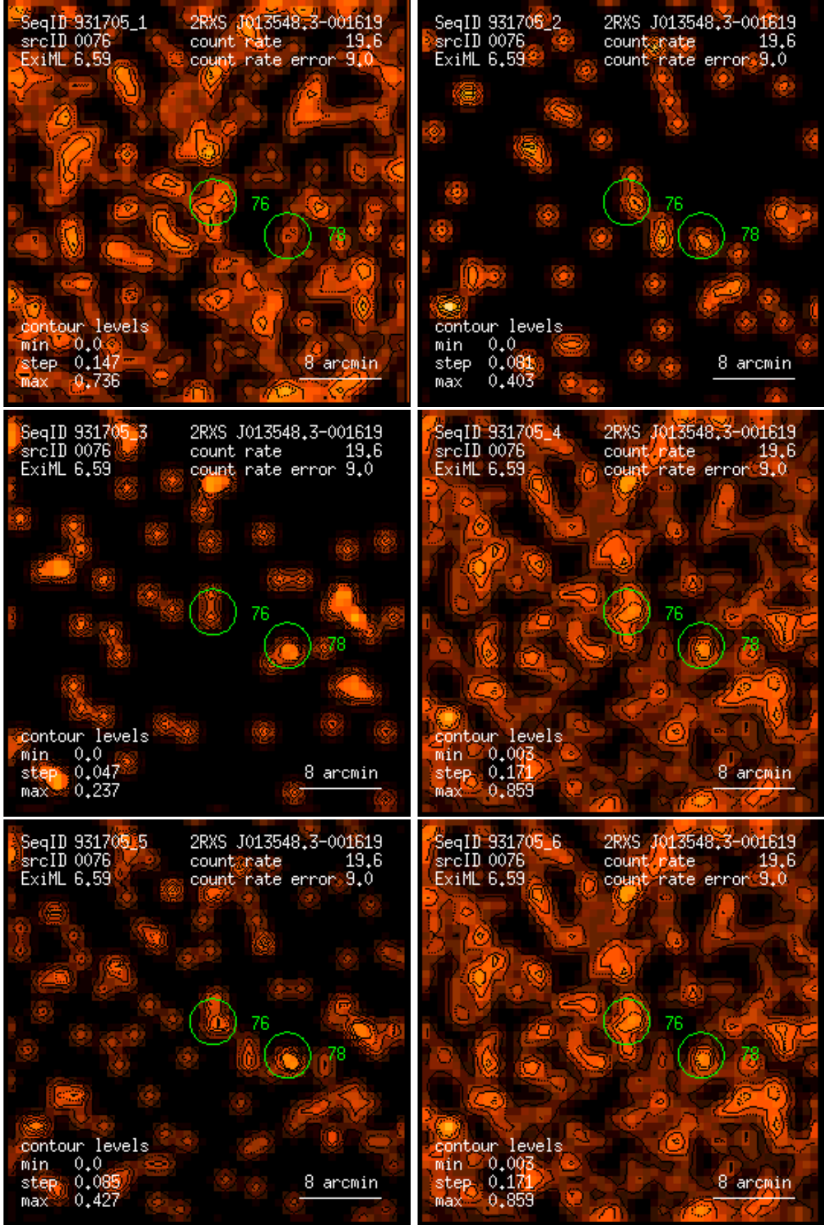
Figure 76: RASS 931705: detection 0076: band rate images, Gaussian filter: (1) PSPC channels 11 – 41, (2) 52 – 90, (3) 91 – 201, (4) 11 – 235, (5) 52 – 201, (6) 11 – 201. Broad band rates in counts/ks. Band rate contour levels in counts/ks/arcmin 2 .
